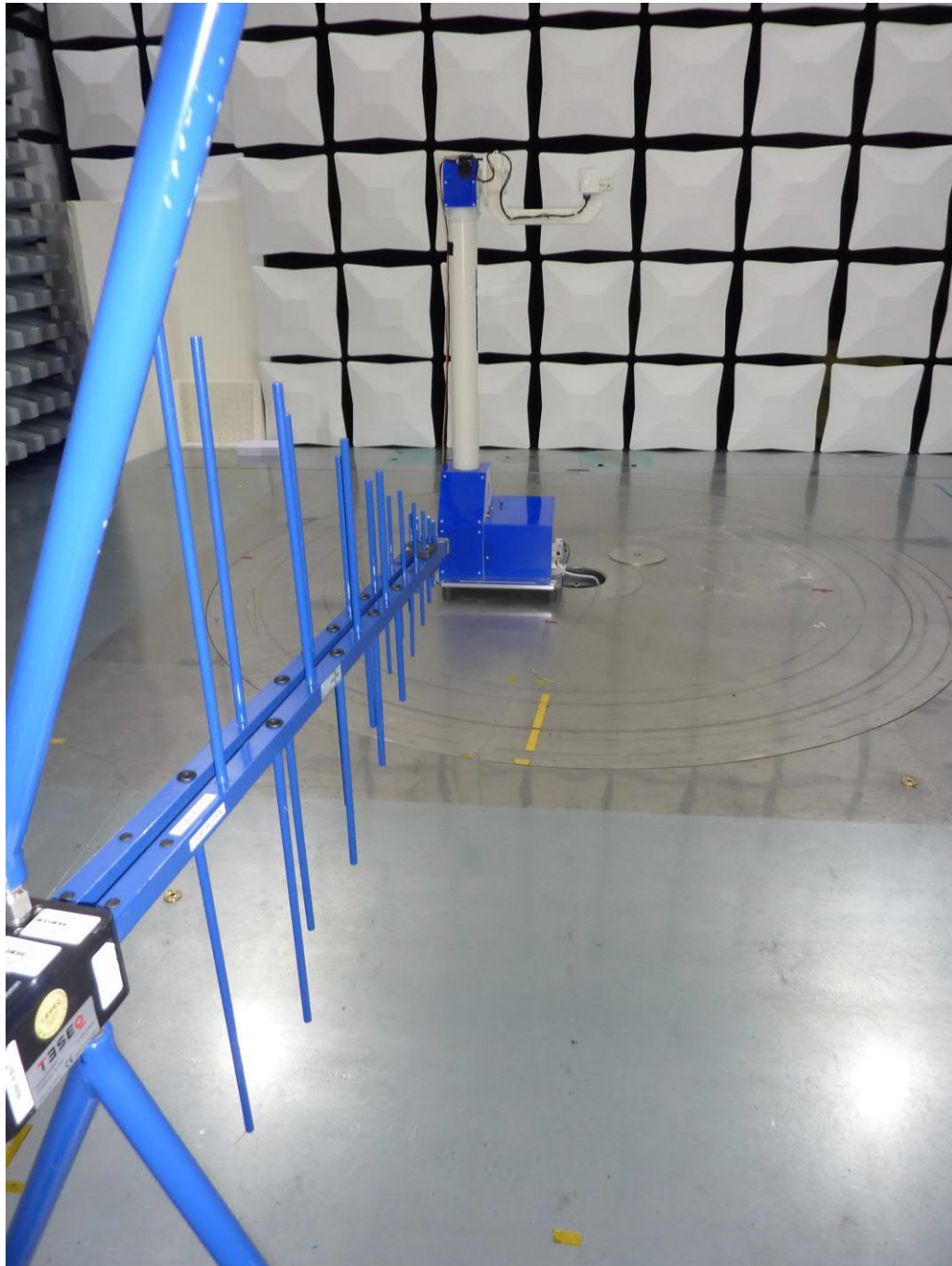
Test setup semi anechoic chamber (variant 1)
