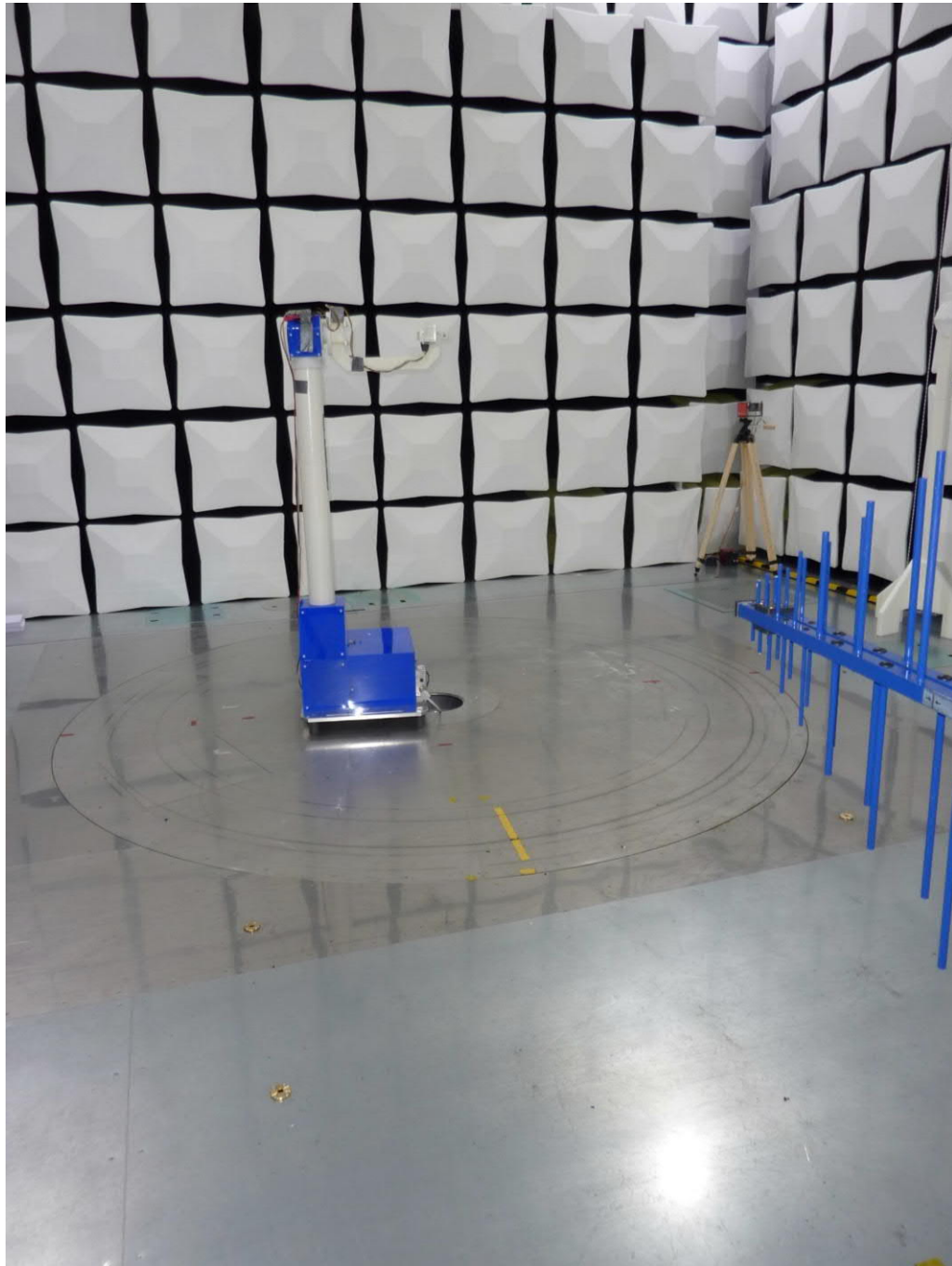
Test setup semi anechoic chamber (variant 4)
