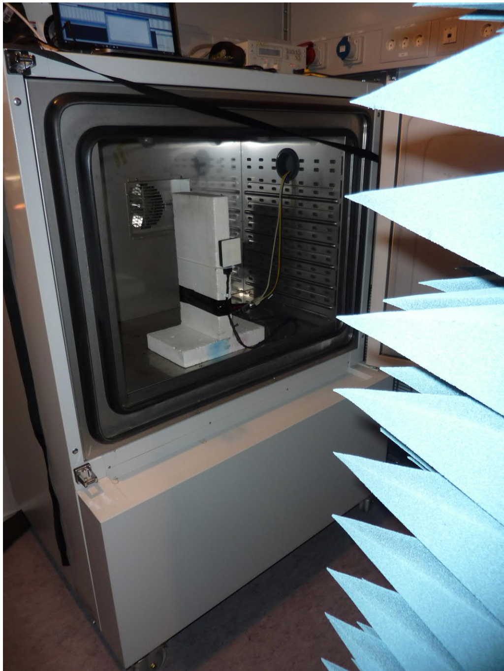
Test setup temperature chamber (isolation removed)
