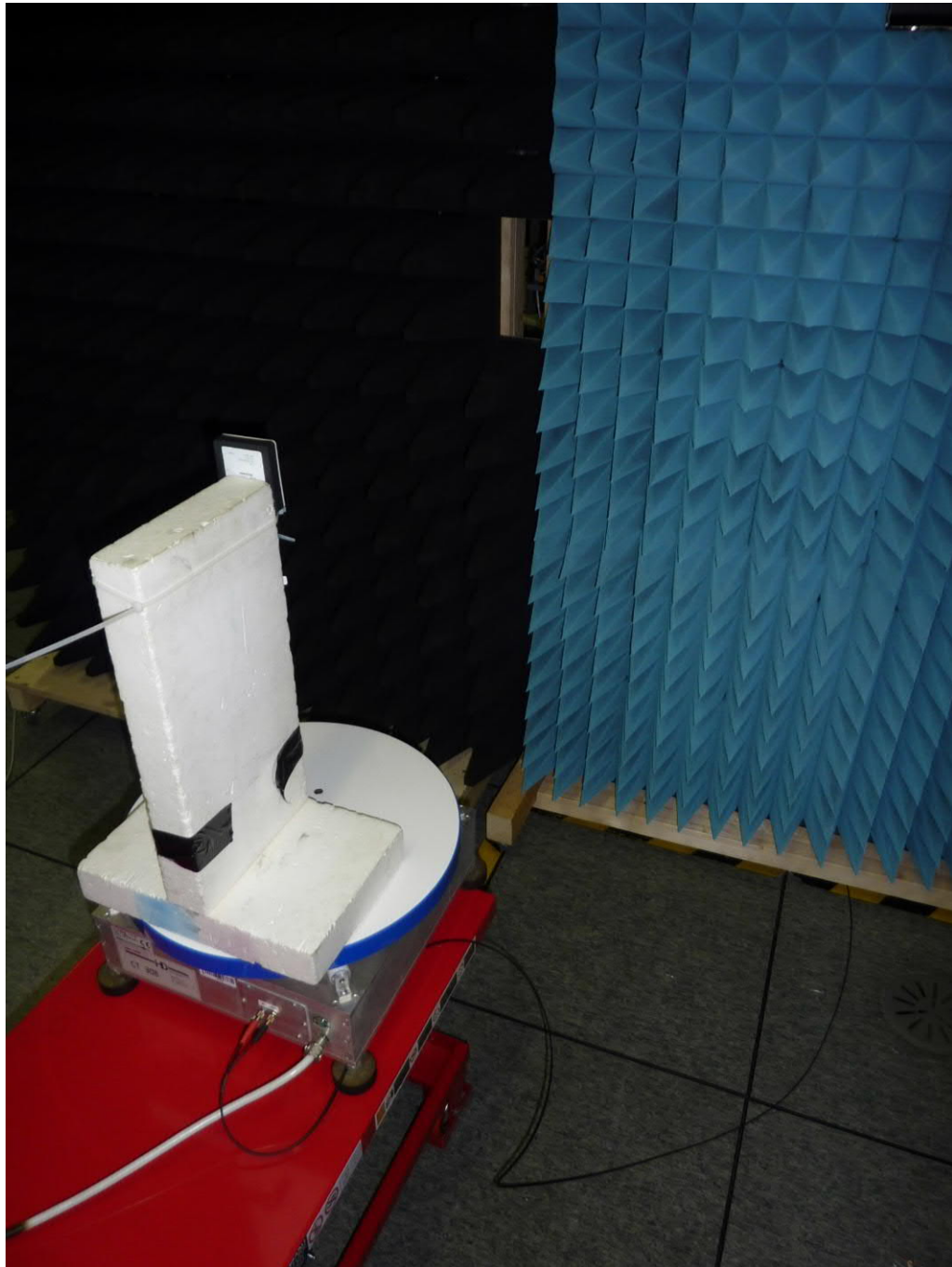
Test setup above 40 GHz
