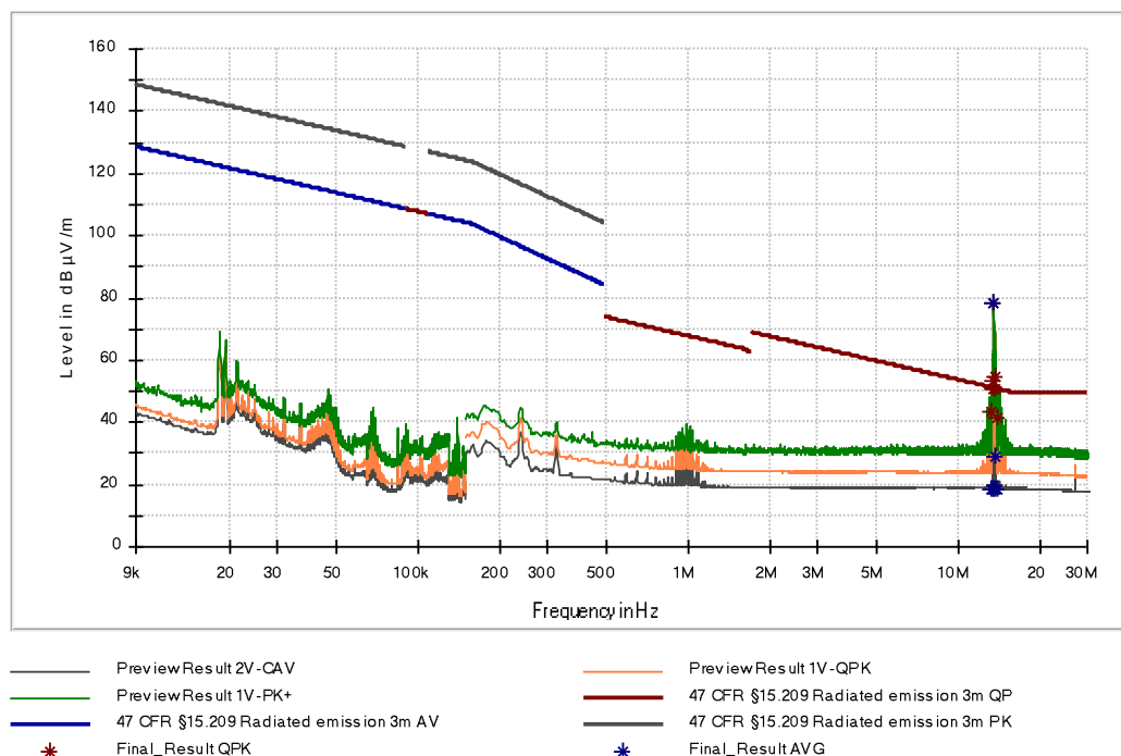
Figure 7: Chart of emissions test below 30 MHz with tag in position 2, antenna in line at 3 m – antenna 2063513:5170
