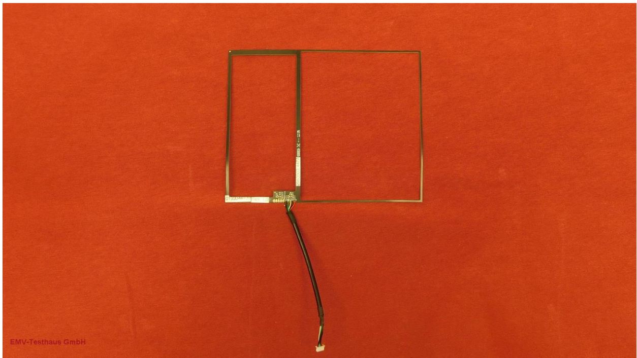
Picture 5: PCB antenna 2063503:4477 small (left half) / large (right half) – top side
