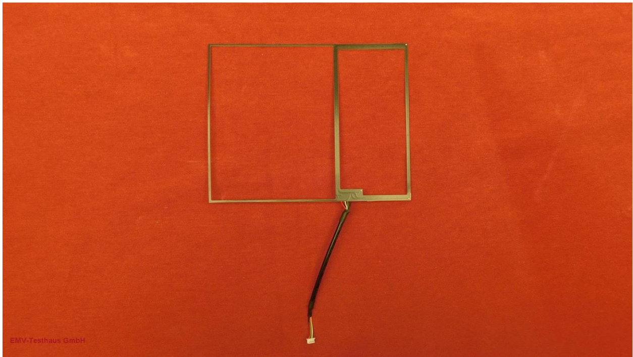
Picture 6: PCB antenna 2063503:4477 small (right half) / large (left half) - bottom side
