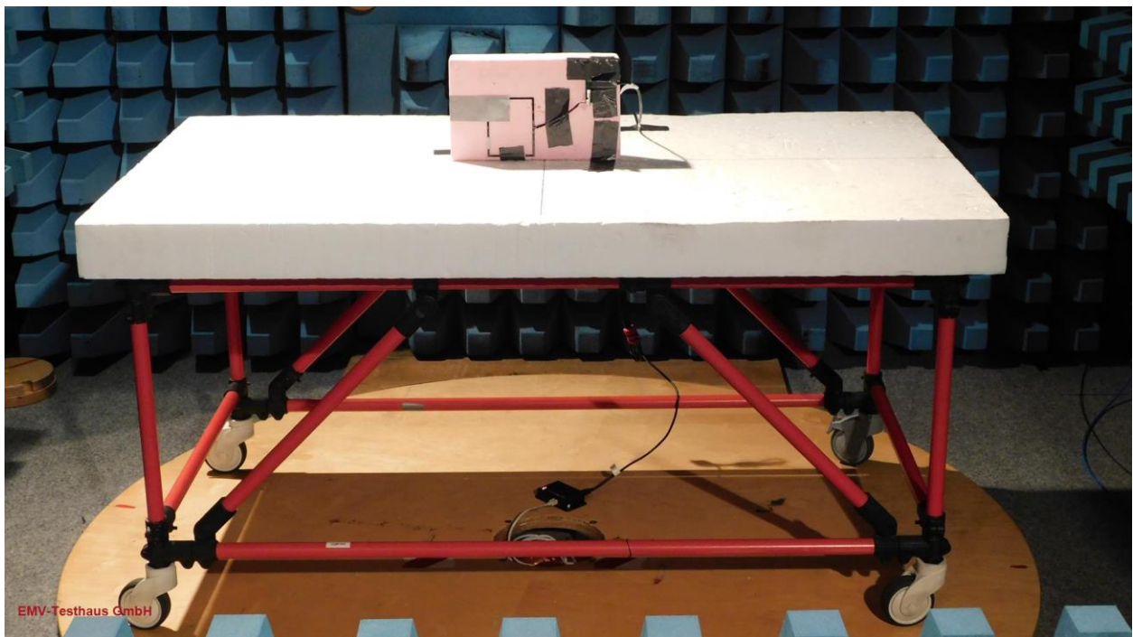
Picture 4: CDC, test setup radiated emission test 9 kHz -30 MHz - PCB antenna 2009168:4834 (rear view)
