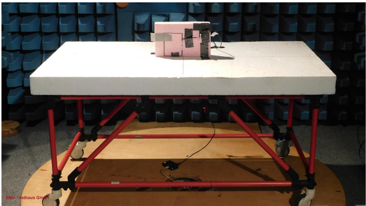
Picture 2: CDC, test setup radiated emission test 9 kHz -30 MHz - PCB antenna 2063512:4612 (rear view)
