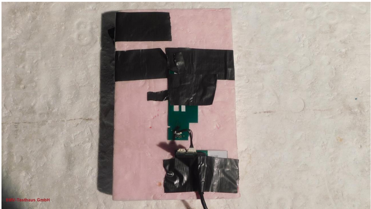
Picture 35: EUT-position 3 - PCB antenna set 2063514:5171
