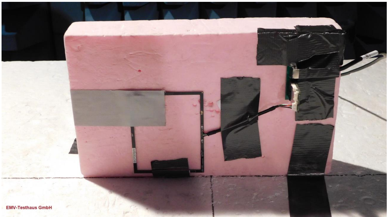
Picture 25: EUT-position 2 - PCB antenna 2009168:4834
