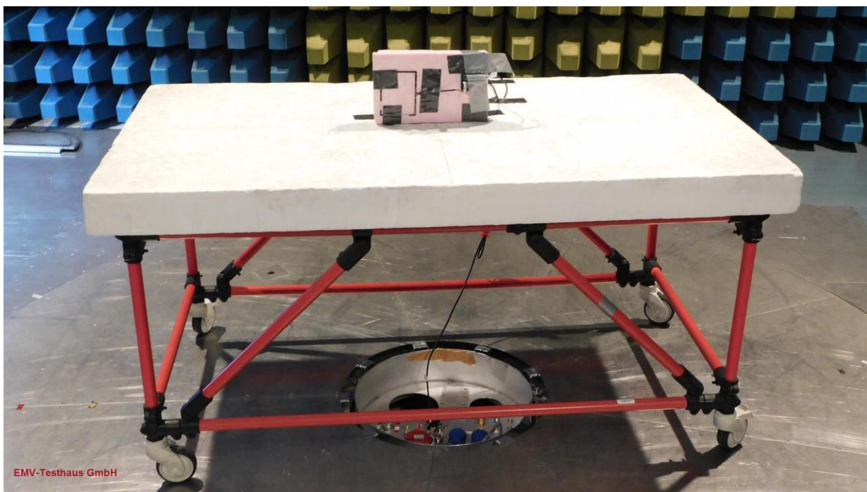
Picture 14: SAC, radiated emission test 30 MHz -1 GHz - PCB antenna 2009168:4834 (rear view)
