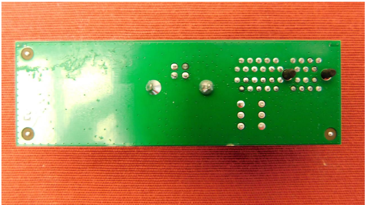
Picture 37: RFID reader module adapter –rear view
