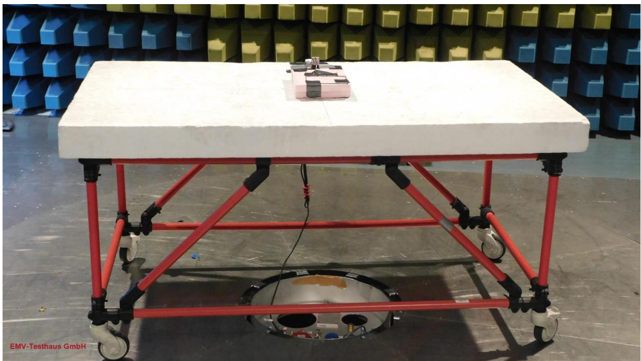
Picture 12: SAC, radiated emission test 30 MHz -1 GHz - PCB antenna 2063512:4612 (rear view)
