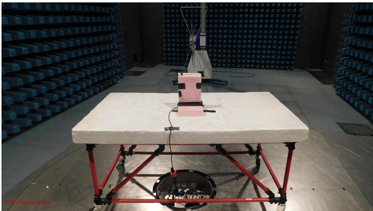
Picture 15: SAC, radiated emission test 30 MHz -1 GHz - PCB antenna set 2063503:4477 (front view)
