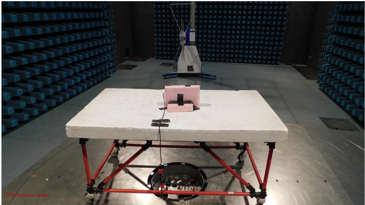
Picture 19: SAC, radiated emission test 30 MHz -1 GHz - PCB antenna 2063514:5171 (front view)
