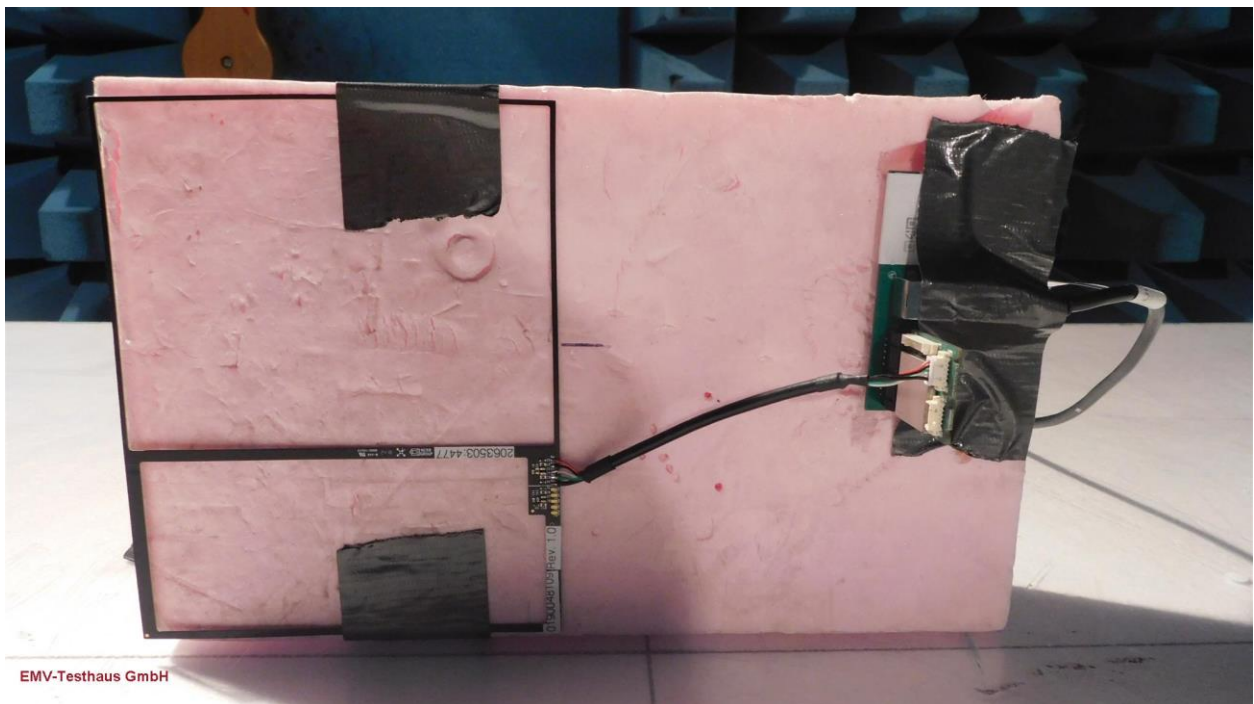
Picture 28: EUT-position 2 - PCB antenna set 2063503:4477
