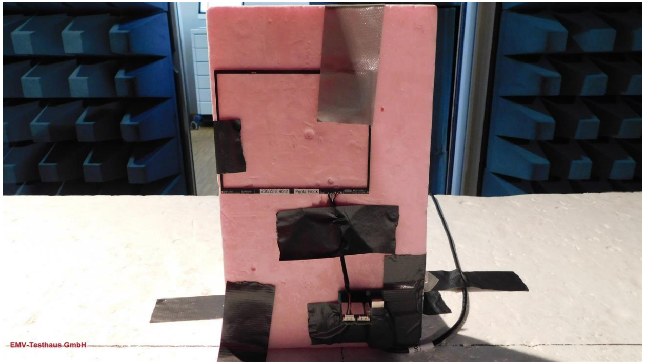
Picture 21: EUT Position 1 - PCB antenna 2063512:4612
