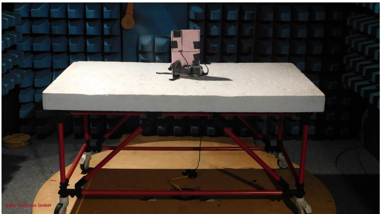
Picture 6: CDC, test setup radiated emission test 9 kHz -30 MHz - PCB antenna set 2063503:4477 (rear view)
