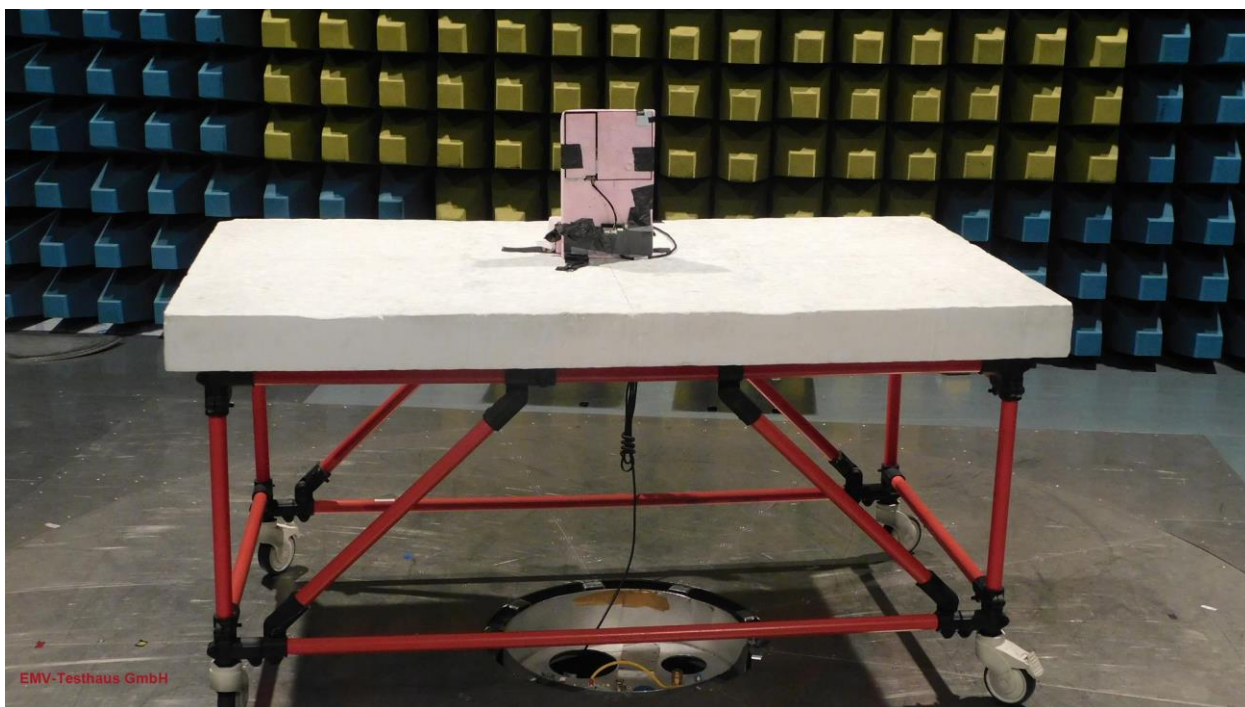
Picture 16: SAC, radiated emission test 30 MHz -1 GHz - PCB antenna set 2063503:4477 (rear view)
