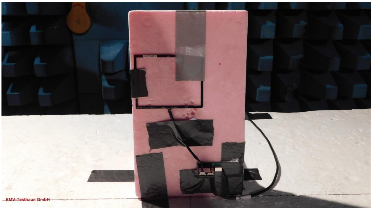
Picture 24: EUT-position 1 - PCB antenna 2009168:4834
