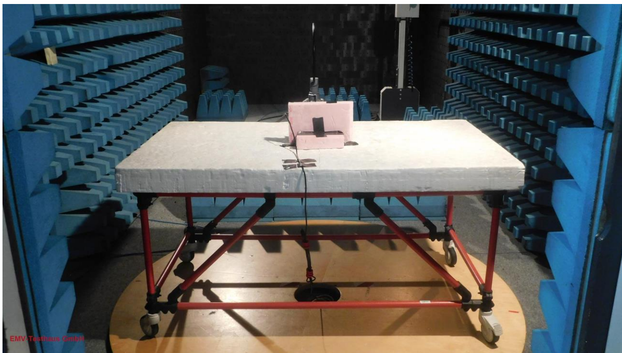
Picture 9: CDC, test setup radiated emission test 9 kHz -30 MHz - PCB antenna 2063514:5171 (front view)
