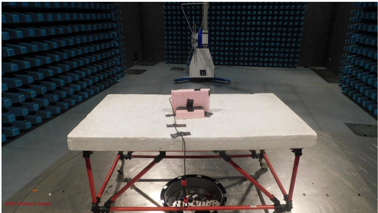
Picture 17: SAC, radiated emission test 30 MHz -1 GHz - PCB antenna 2063513:5170 (front view)
