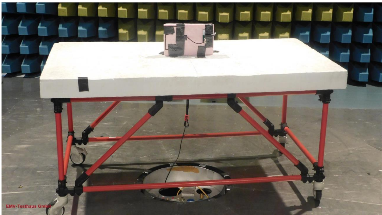
Picture 18: SAC, radiated emission test 30 MHz -1 GHz - PCB antenna 2063513:5170 (rear view)
