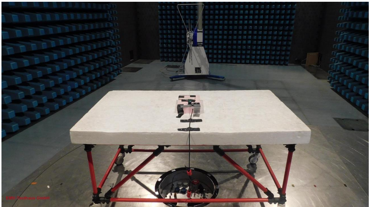
Picture 11: SAC, radiated emission test 30 MHz -1 GHz - PCB antenna 2063512:4612 (front view)
