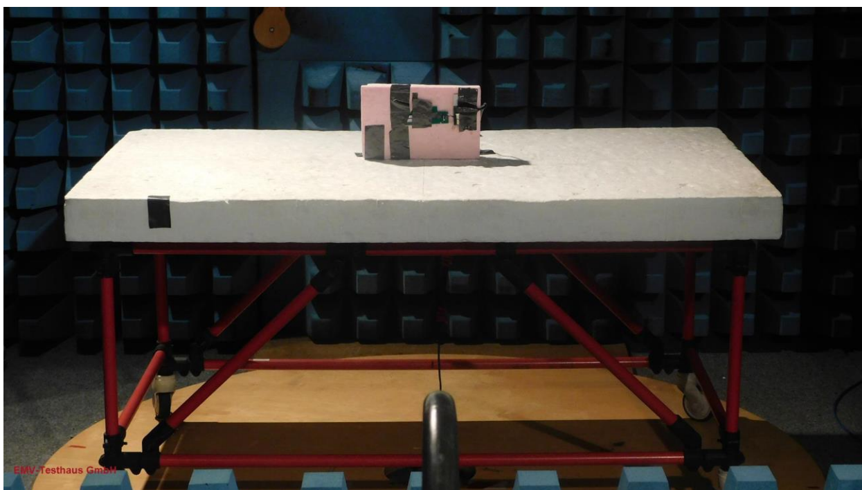
Picture 10: CDC, test setup radiated emission test 9 kHz -30 MHz - PCB antenna set 2063514:5171 (rear view)
