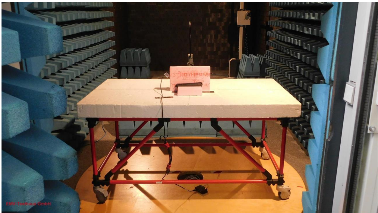
Picture 1: CDC, test setup radiated emission test 9 kHz -30 MHz - PCB antenna 2063512:4612 (front view)
