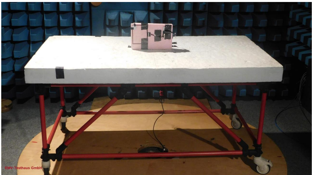
Picture 8: CDC, test setup radiated emission test 9 kHz -30 MHz - PCB antenna set 2063513:5170 (rear view)
