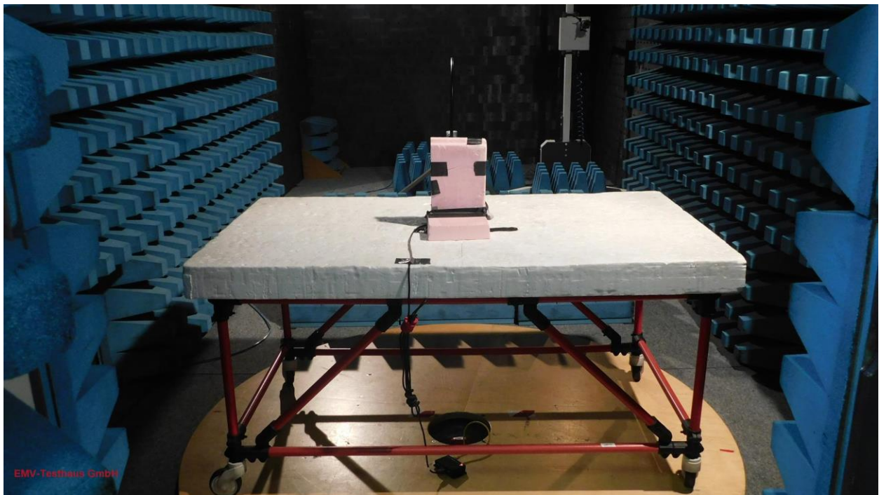
Picture 5: CDC, test setup radiated emission test 9 kHz -30 MHz - PCB antenna set 2063503:4477 (front view)
