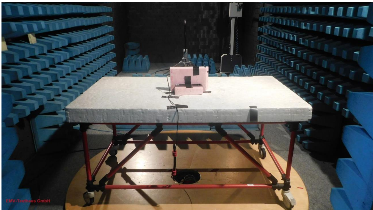
Picture 7: CDC, test setup radiated emission test 9 kHz -30 MHz - PCB antenna 2063513:5170 (front view)
