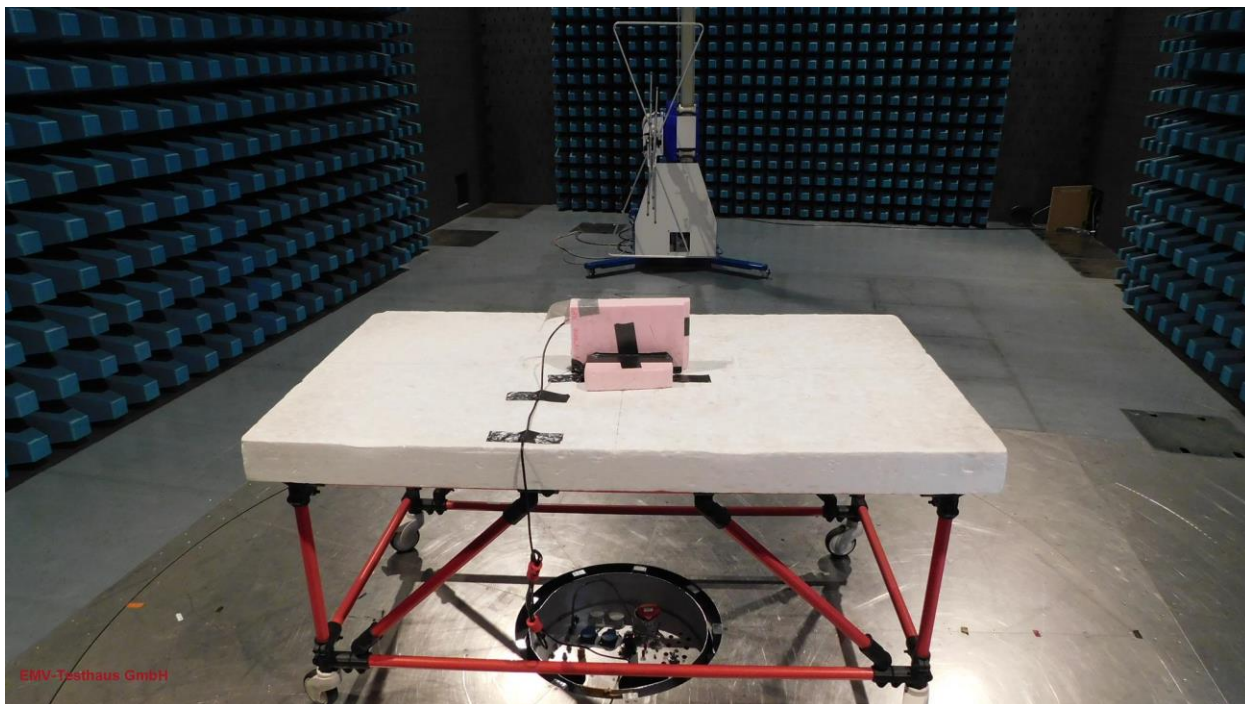
Picture 13: SAC, radiated emission test 30 MHz -1 GHz - PCB antenna 2009168:4834 (front view)
