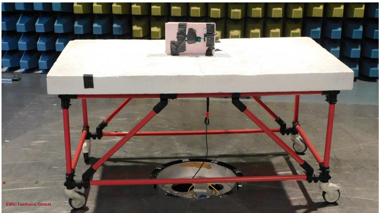
Picture 20: SAC, radiated emission test 30 MHz -1 GHz - PCB antenna 2063514:5171 (rear view)
