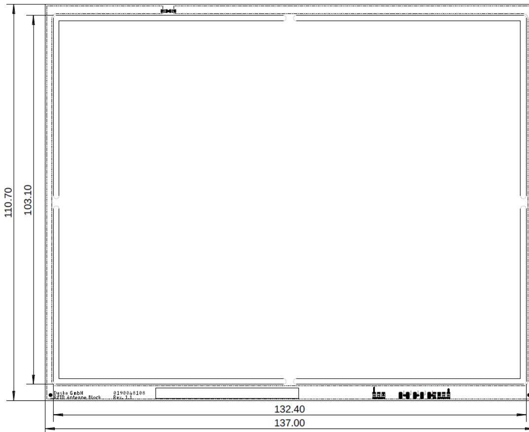
Antenna Penta Block: Depth = 1.66mm
