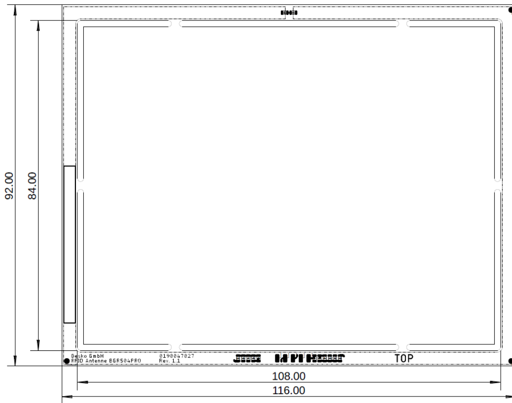
Antenna BGR504pro: Depth = 1.27 mm
