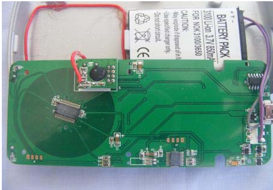
internal construction detail (back)
