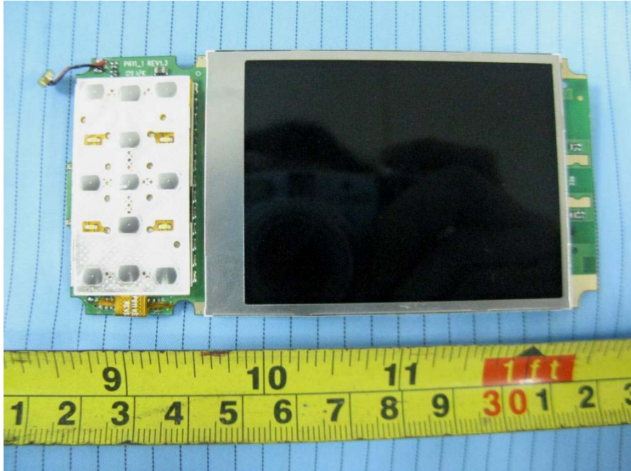
EUT – Main Board Top moved LCD and Keyboard View
