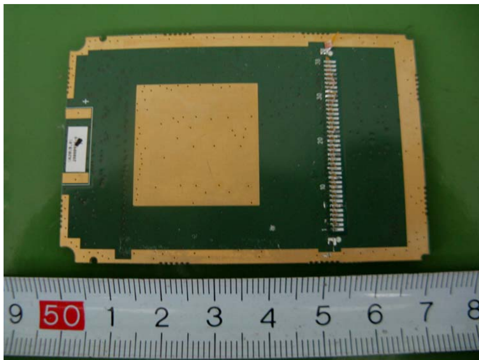
EUT – LCD Board U620UB Bottom View
