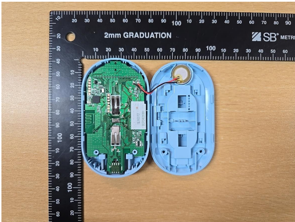
< Cover open >
