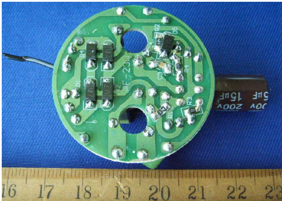
EUT–Solder View (HLFR15W)
