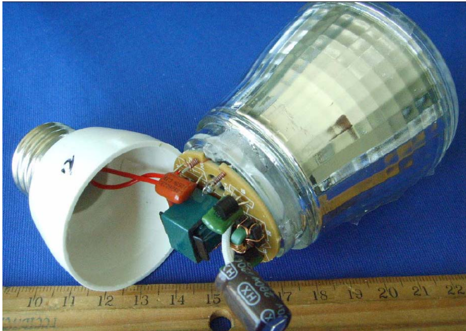
EUT –Components View (HLFR11W)
