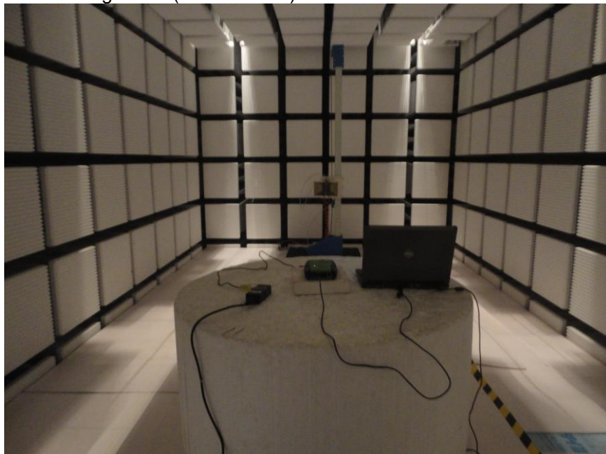
Transmitting mode (Above 1GHz)
