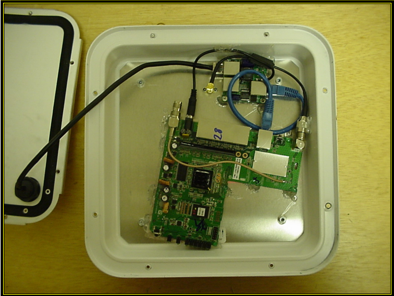
Photograph 5: Inside with PCB and Antenna
