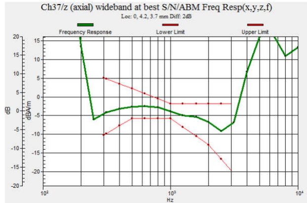
Fig 7.2 GSM900 Ch37
