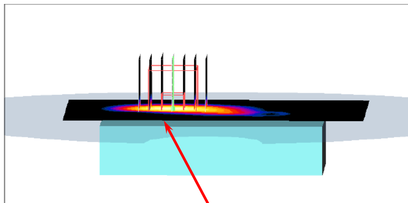
Figure 9. Body SAR Test Setup (Flat Section) _ Front Surface
