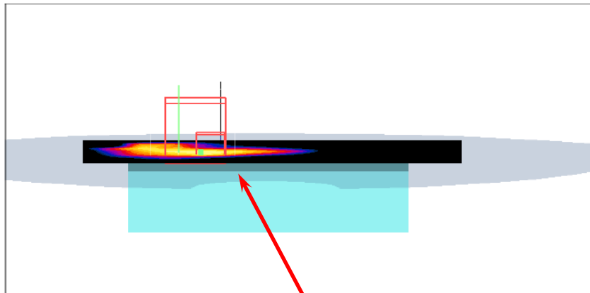
Figure 10. Body SAR Test Setup (Flat Section) _ Back Surface
