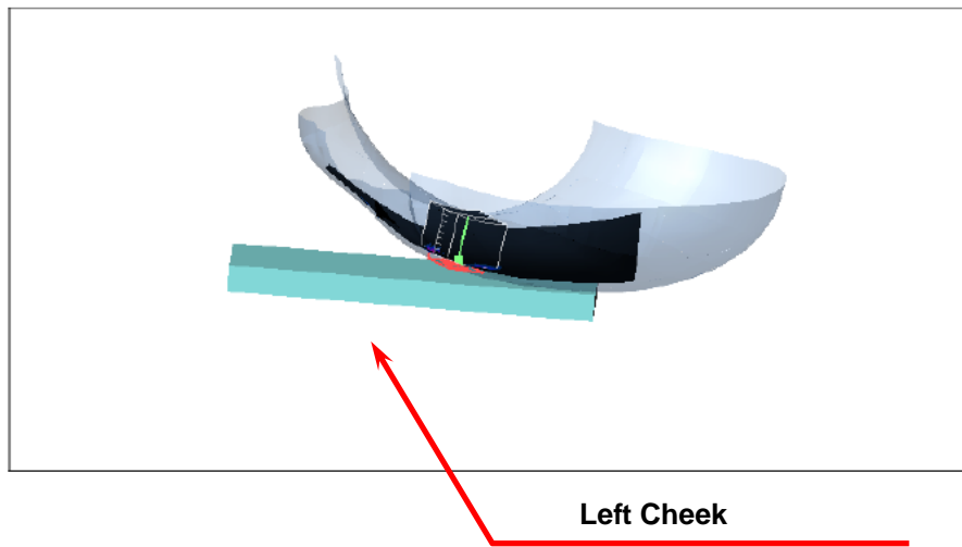
Figure 6. Left Head SAR Test Setup (Cheek)
