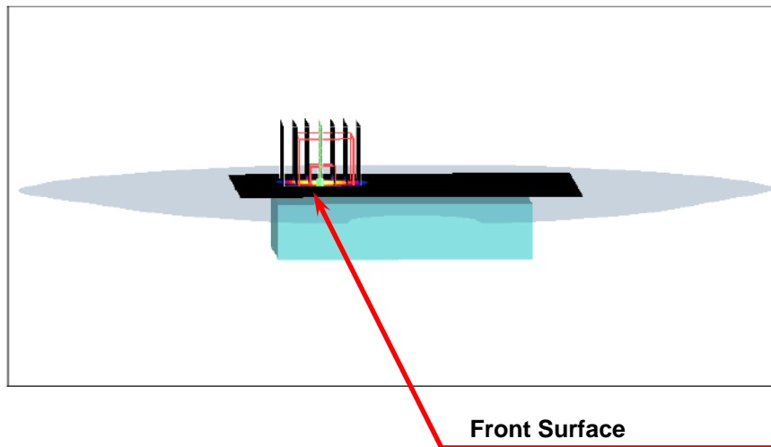
Figure 7. Body SAR Test Setup (Flat Section) _ Front Surface
