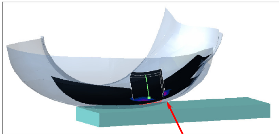
Figure 3. Right Head SAR Test Setup (Cheek)
