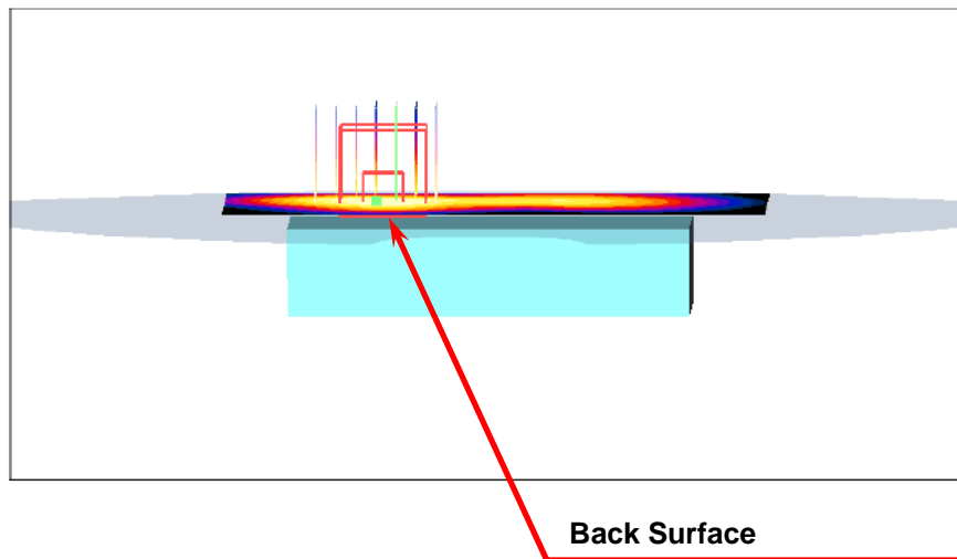
Figure 8. Body SAR Test Setup (Flat Section) _ Back Surface
