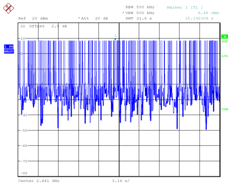
Fig.54 Time of occupancy (Dwell Time): Ch39,Packet 2-DH3
