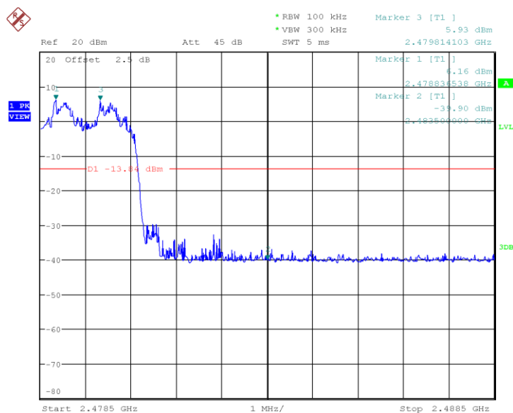
Fig.20 Frequency Band Edge: 8DPSK, Ch78, Hopping OFF
