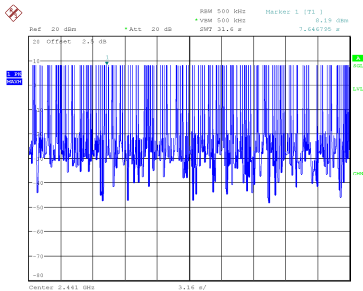
Fig.60 Time of occupancy (Dwell Time): Ch39,Packet 3-DH3
