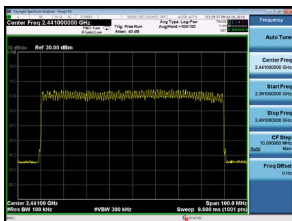
3DH5 2400 MHz – 2483.5 MHz
