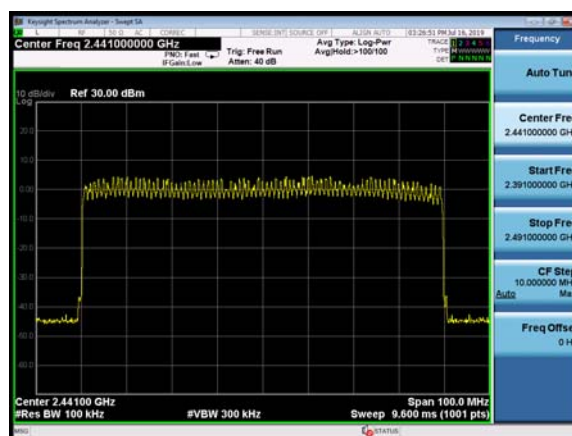
2DH5 2400 MHz – 2483.5 MHz
