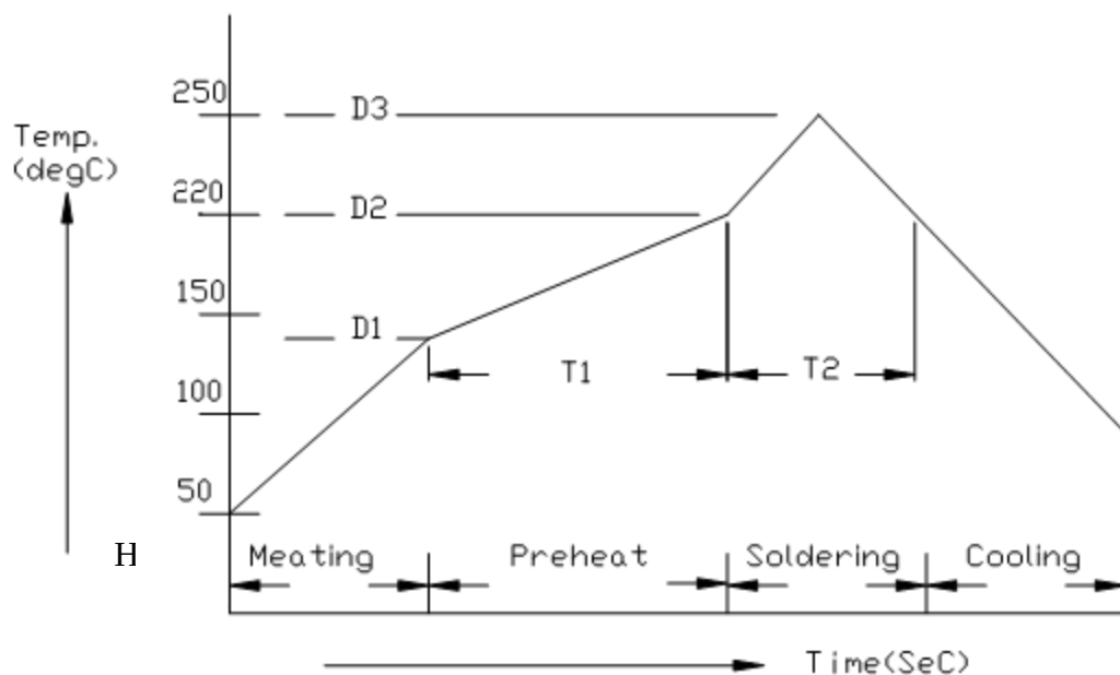
Figure 15 – Reflow profile
