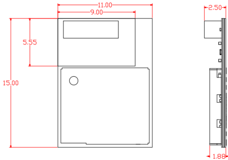
Figure 13 – Module Mechanical Outline (TOP and Side View)
