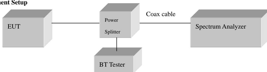
Figure 1: Measurement setup for the carrier frequency separation
