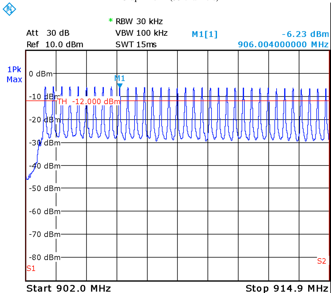
Graph 1 of 2 (35 channels)
