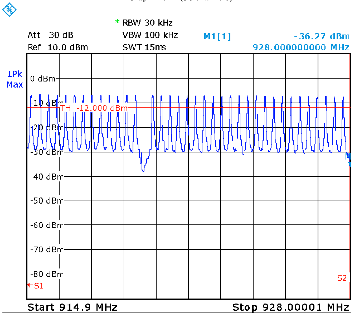
Graph 2 of 2 (36 channels)
