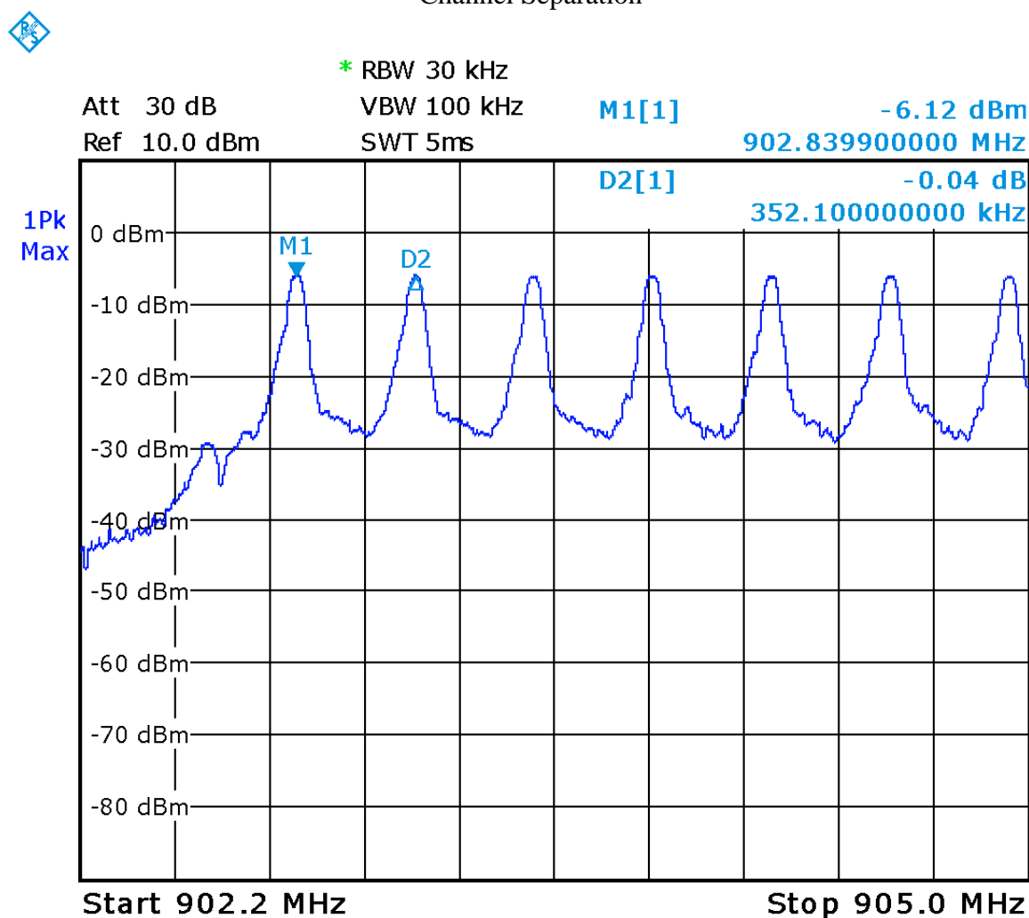
Channel Separation
