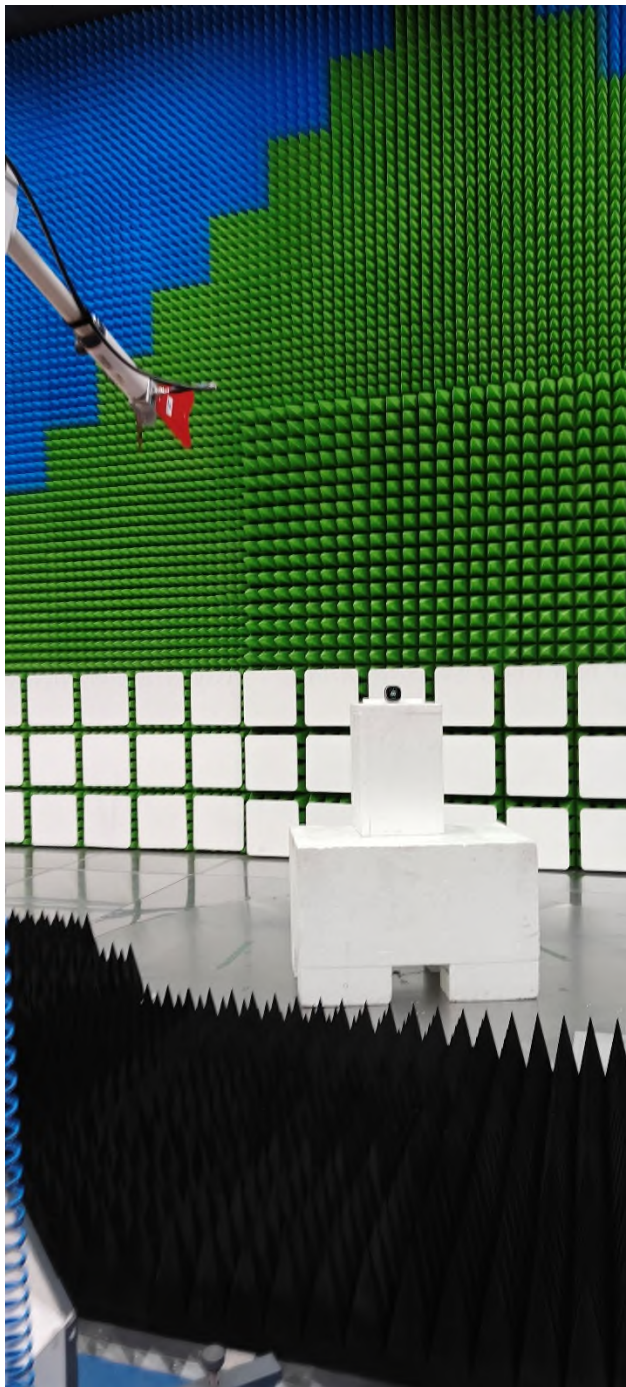
Figure 4 – Radiated Emissions Setup 1GHz – 18GHz
