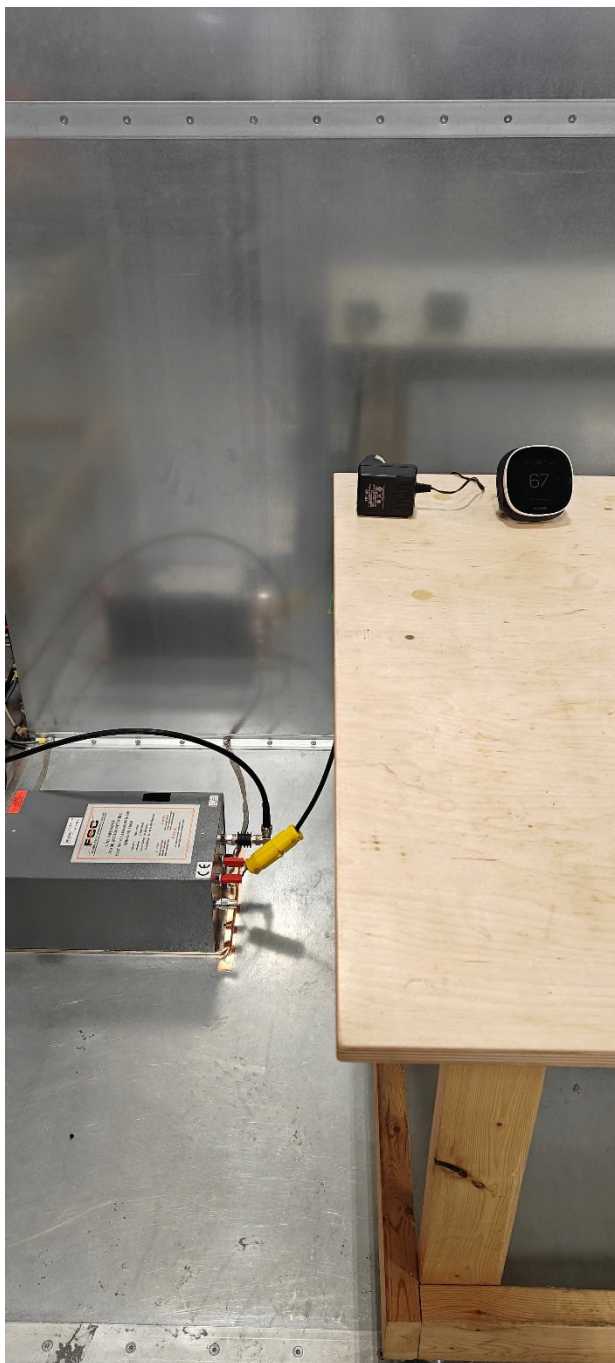
Figure 5 – Conducted Emissions Setup
