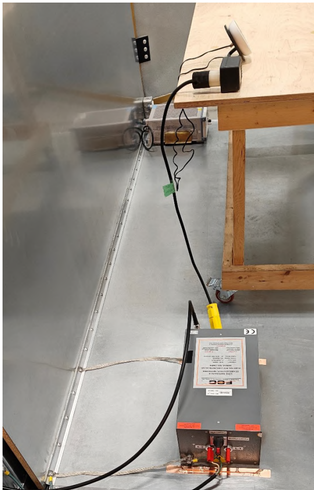
Figure 6 – Conducted Emissions Setup
