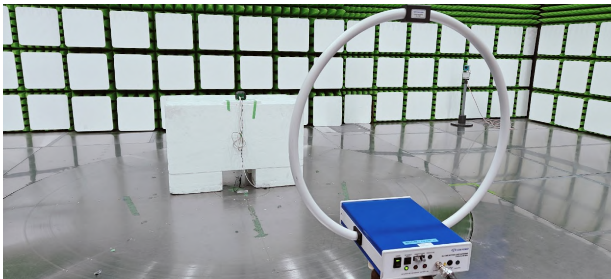
Figure 2 – Radiated Emissions Setup 9kHz – 30MHz
