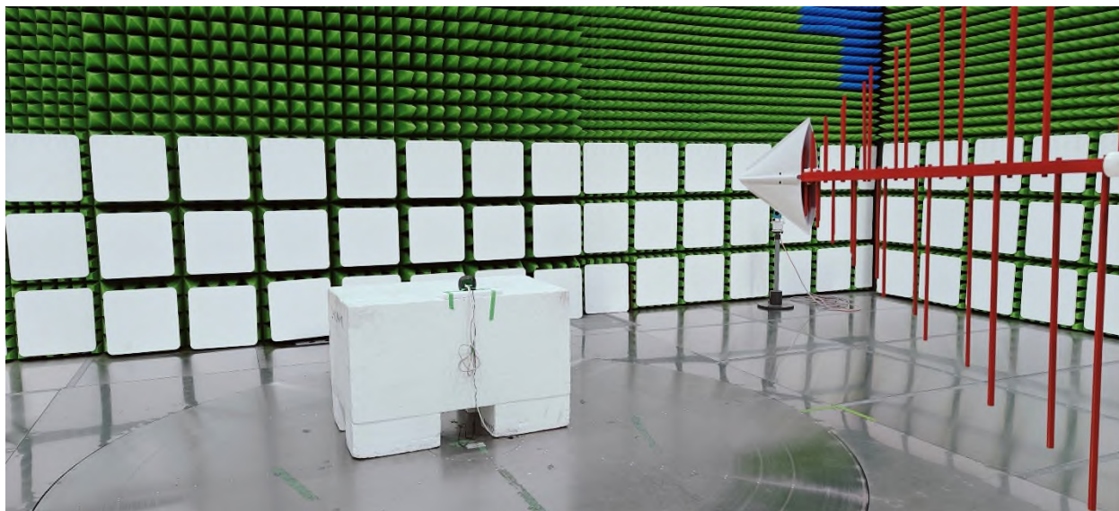
Figure 3 – Radiated Emissions Setup 30MHz – 1GHz
