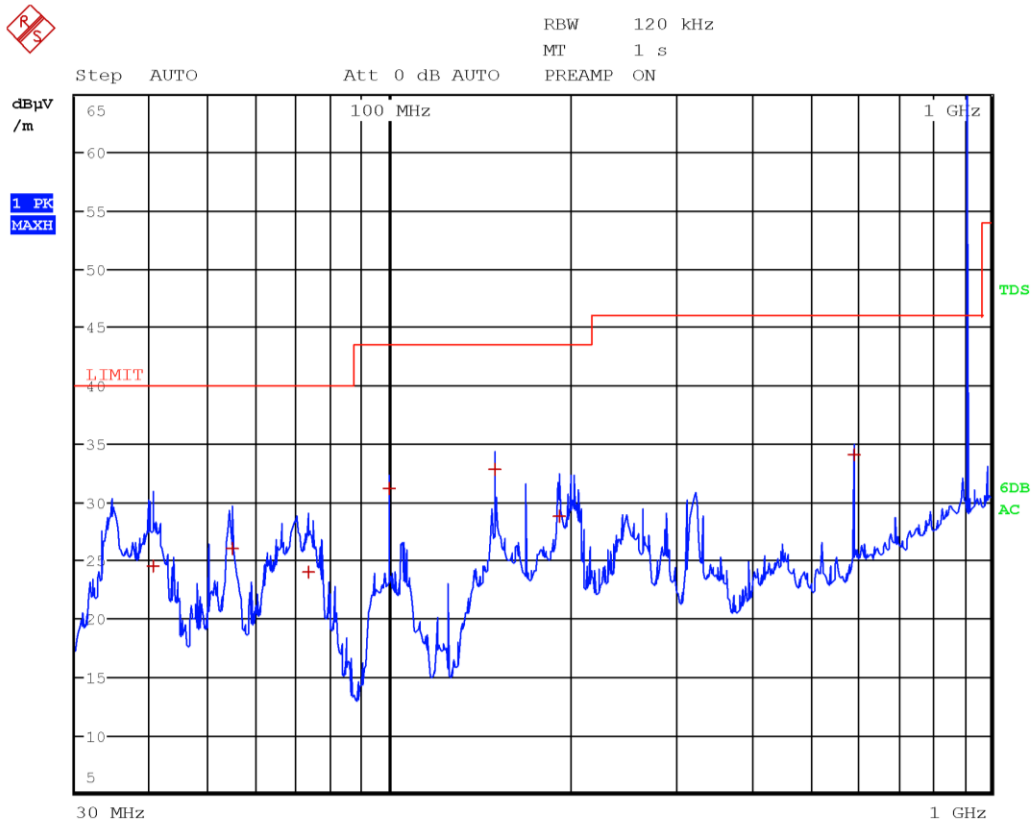
Radiated spurious emissions with antenna in vertical polarization and with LTE Tx at 1732.5 MHz, UHF Tx at 915 MHz, WIFI Tx at 2437 MHz and BT Tx at 2441 MHz (antenna configuration 1)
