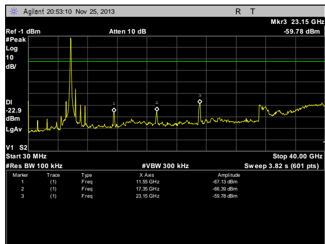
Plot 21. Conducted Spurious Emissions, Channel 149, Chain 1, 30 MHz – 40 GHz
