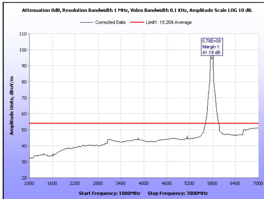
Plot 17. Radiated Spurious Emissions, Channel 149, 1 GHz – 7 GHz, Average
