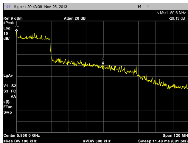
Plot 28. Conducted Band Edge, High, Channel 149, Chain 2
