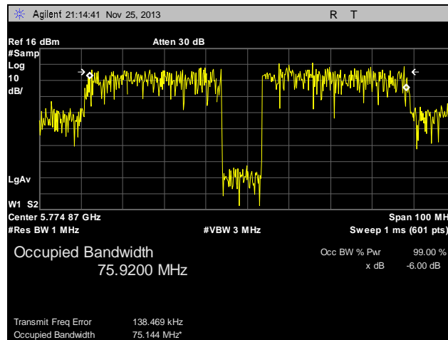
Plot 10. 99% Occupied Bandwidth, Channel 149, Chain 0
