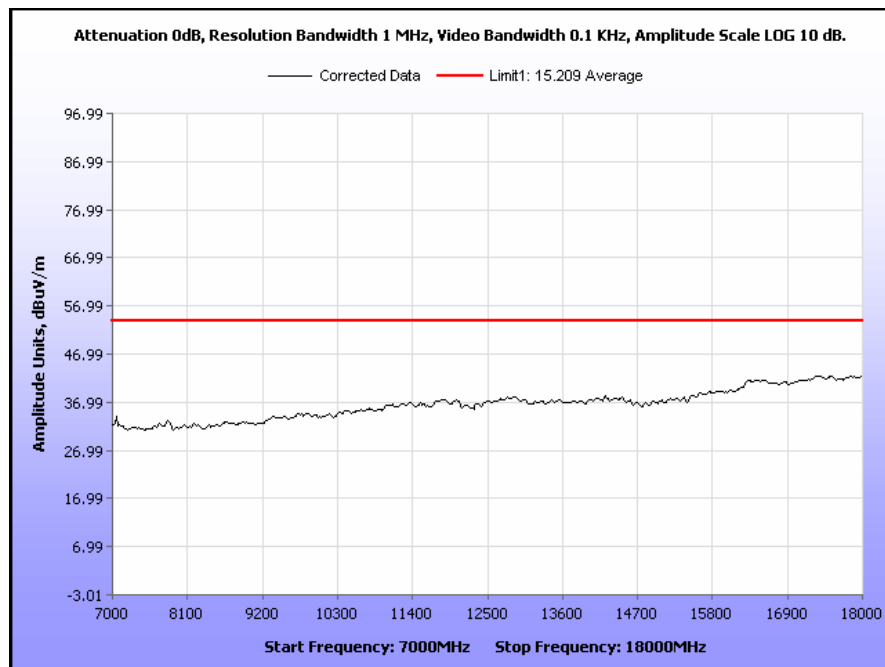
Plot 19. Radiated Spurious Emissions, Channel 149, 7 GHz – 18 GHz, Average
