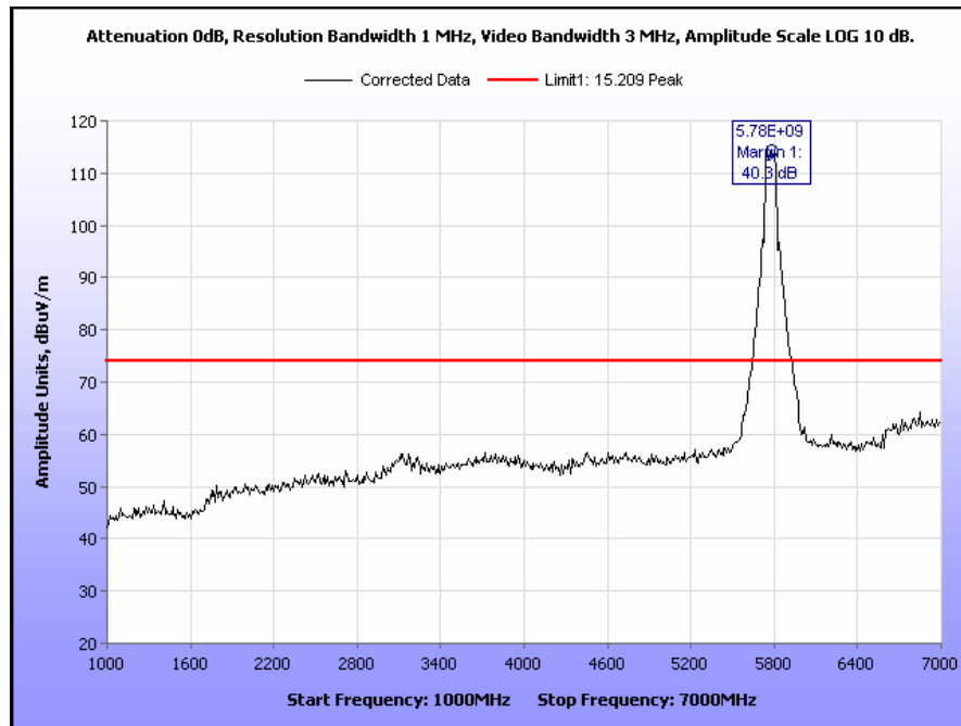
Plot 16. Radiated Spurious Emissions, Channel 149, 1 GHz – 7 GHz, Peak
