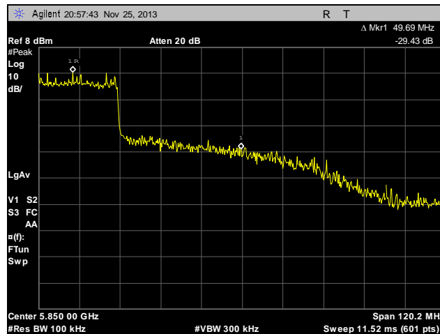
Plot 27. Conducted Band Edge, High, Channel 149, Chain 1
