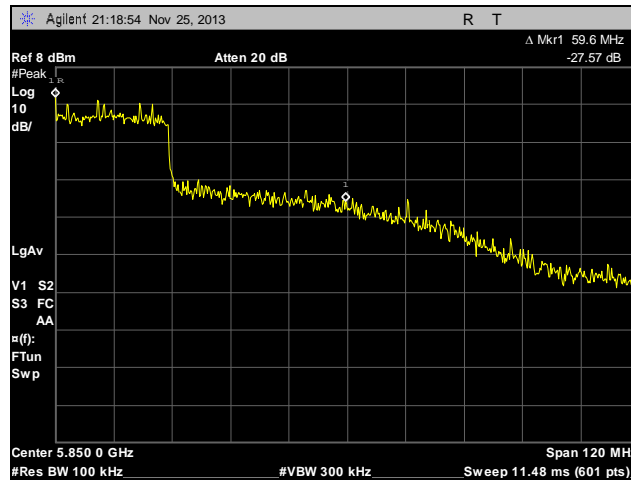
Plot 26. Conducted Band Edge, High, Channel 149, Chain 0
