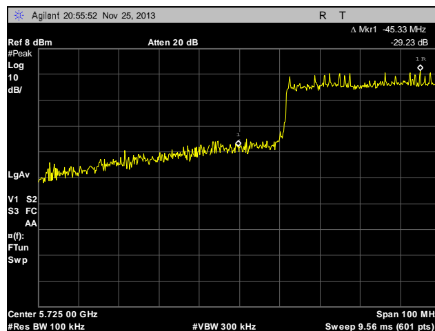
Plot 24. Conducted Band Edge, Low, Channel 149, Chain 1
