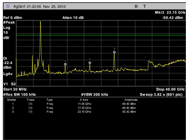
Plot 20. Conducted Spurious Emissions, Channel 149, Chain 0, 30 MHz – 40 GHz
