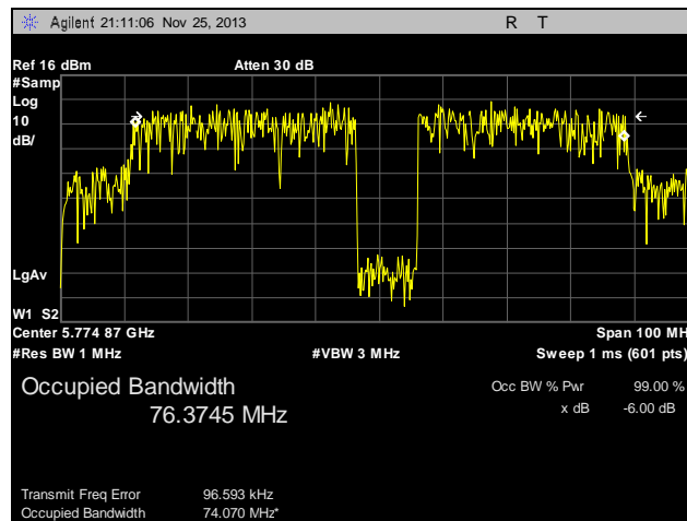
Plot 11. 99% Occupied Bandwidth, Channel 149, Chain 1
