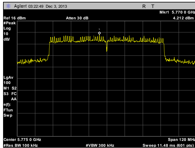
Plot 29. Peak Power Spectral Density, Channel 149, Chain 0
