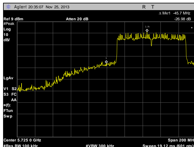
Plot 25. Conducted Band Edge, Low, Channel 149, Chain 2
