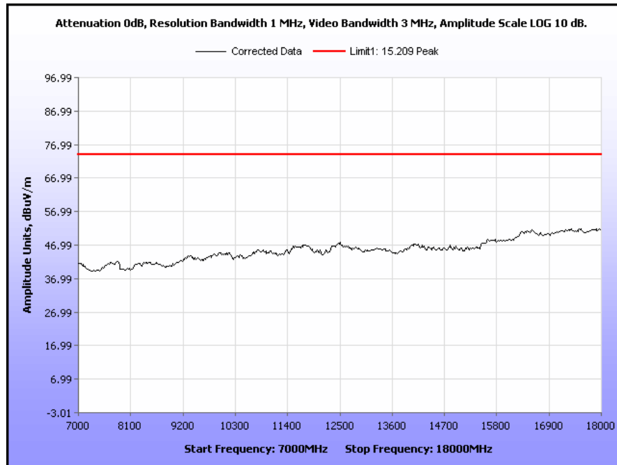
Plot 18. Radiated Spurious Emissions, Channel 149, 7 GHz – 18 GHz, Peak
