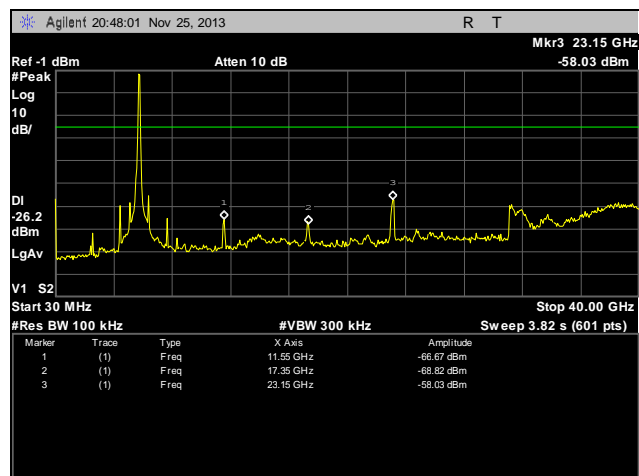
Plot 22. Conducted Spurious Emissions, Channel 149, Chain 2, 30 MHz – 40 GHz
