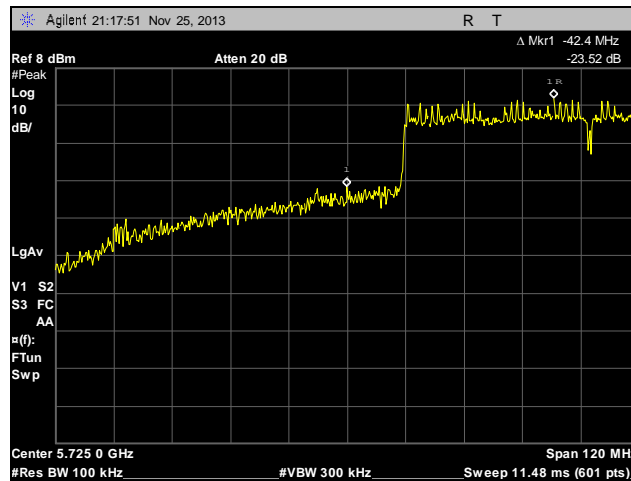
Plot 23. Conducted Band Edge, Low, Channel 149, Chain 0
