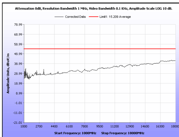
Plot 27. Radiated Spurious Emissions, Low Channel, 802.11n 20 MHz, 1 GHz – 18 GHz, Average
