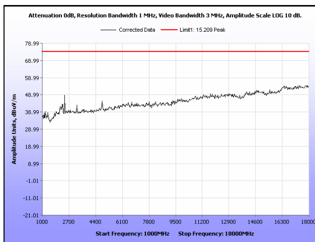
Plot 26. Radiated Spurious Emissions, Low Channel, 802.11n 20 MHz, 1 GHz – 18 GHz, Peak
