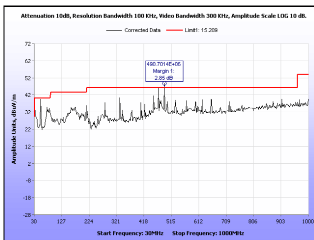
Plot 13. Radiated Spurious Emissions, High Channel, 802.11b, 30 MHz – 1 GHz
