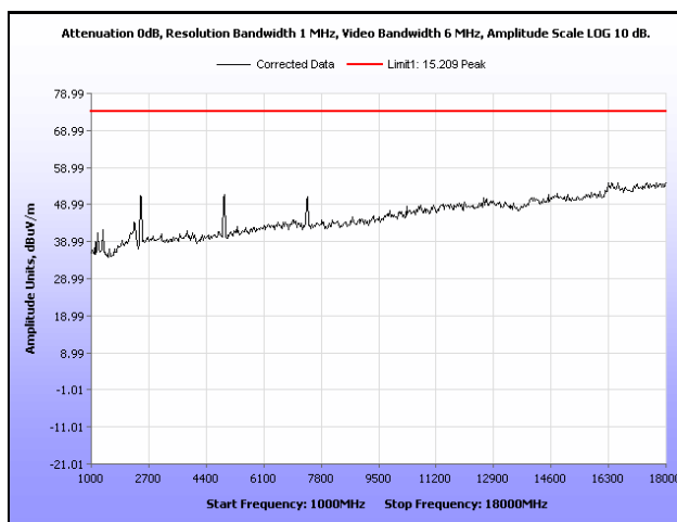
Plot 23. Radiated Spurious Emissions, High Channel, 802.11g, 1 GHz – 18 GHz, Peak
