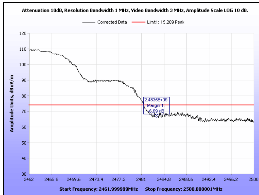
Plot 46. Radiated Restricted Band Edge, 802.11b, High Channel, Peak
