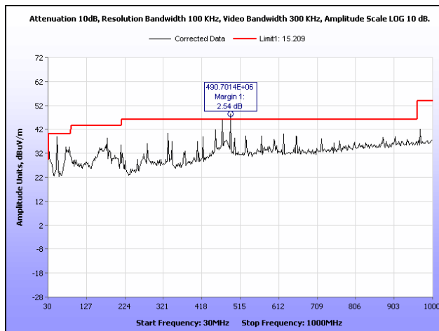
Plot 19. Radiated Spurious Emissions, Mid Channel, 802.11g, 30 MHz – 1 GHz
