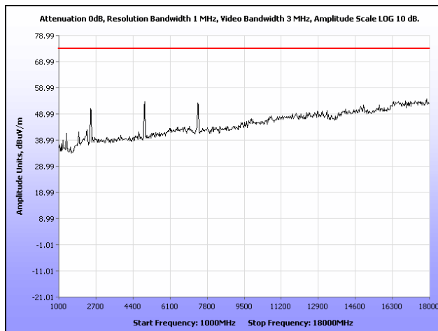
Plot 14. Radiated Spurious Emissions, High Channel, 802.11b, 1 GHz – 18 GHz, Peak
