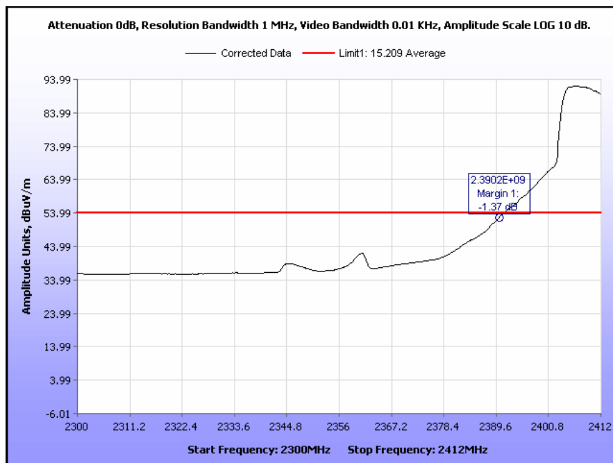
Plot 51. Radiated Restricted Band Edge, 802.11n 20 MHz, Low Channel, Average
