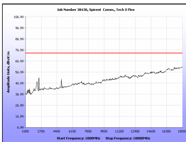
Plot 29. Radiated Spurious Emissions, Mid Channel, 802.11n 20 MHz, 1 GHz – 18 GHz, Peak
