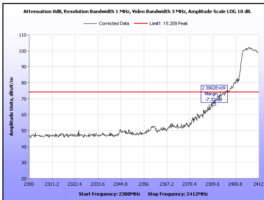
Plot 52. Radiated Restricted Band Edge, 802.11n 20 MHz, Low Channel, Peak
