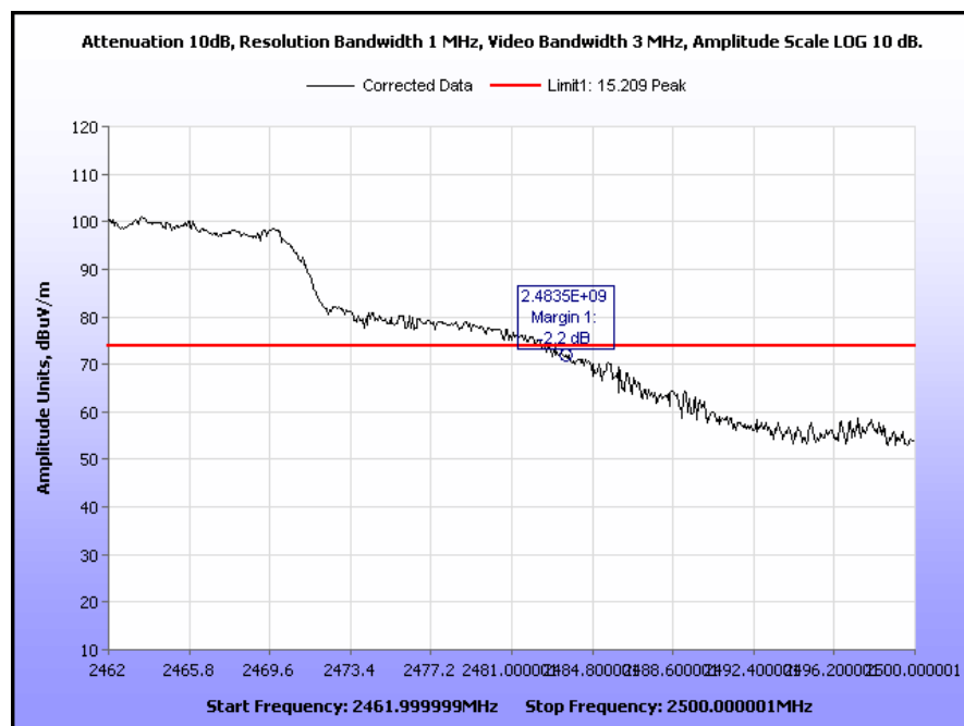
Plot 50. Radiated Restricted Band Edge, 802.11g, High Channel, Peak
