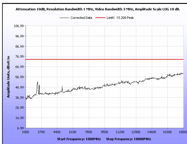
Plot 41. Radiated Spurious Emissions, High Channel, 802.11n 40 MHz, 1 GHz – 18 GHz, Peak
