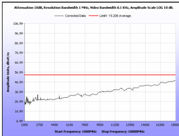
Plot 33. Radiated Spurious Emissions, High Channel, 802.11n 20 MHz, 1 GHz – 18 GHz, Average
