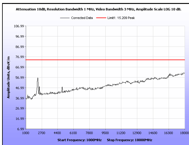
Plot 38. Radiated Spurious Emissions, Mid Channel, 802.11n 40 MHz, 1 GHz – 18 GHz, Peak
