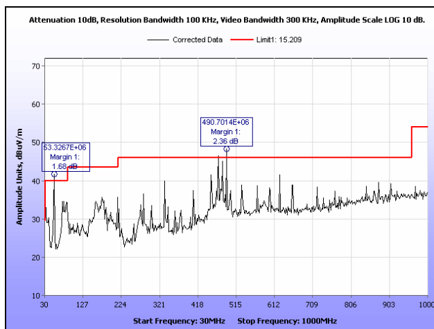
Plot 28. Radiated Spurious Emissions, Mid Channel, 802.11n 20 MHz, 30 MHz – 1 GHz
