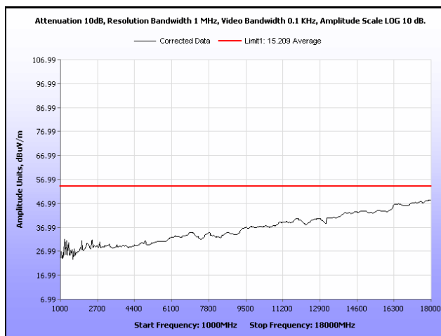
Plot 39. Radiated Spurious Emissions, Mid Channel, 802.11n 40 MHz, 1 GHz – 18 GHz, Average
