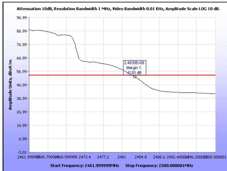
Plot 49. Radiated Restricted Band Edge, 802.11g, High Channel, Average
