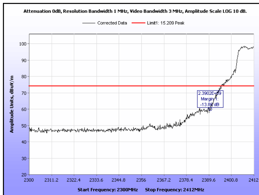
Plot 48. Radiated Restricted Band Edge, 802.11g, Low Channel, Peak
