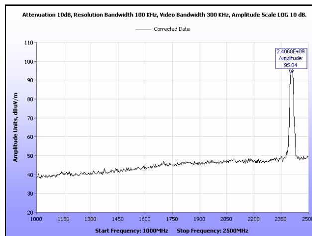
Plot 7. Radiated Spurious Emissions, Low Channel, 802.11b, Above 1 GHz, Fundamental Marked
