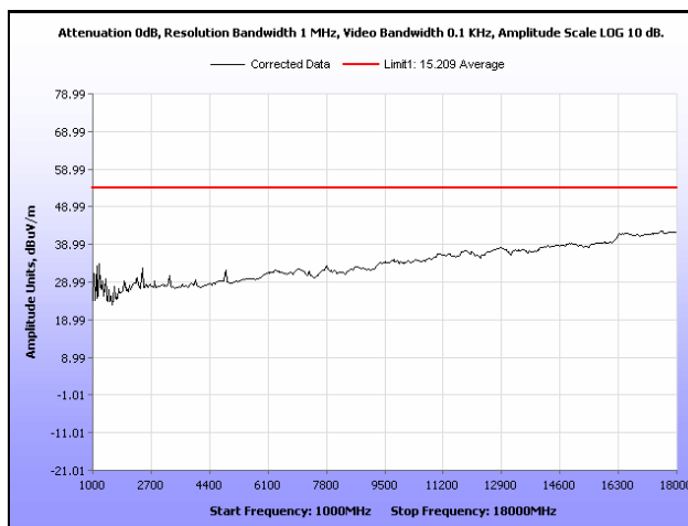
Plot 24. Radiated Spurious Emissions, High Channel, 802.11g, 1 GHz – 18 GHz, Average
