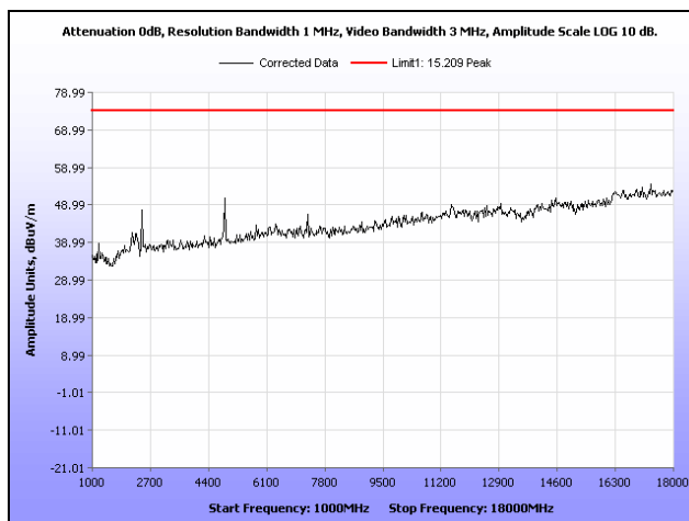
Plot 11. Radiated Spurious Emissions, Mid Channel, 802.11b, 1 GHz – 18 GHz, Peak
