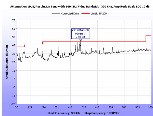
Plot 22. Radiated Spurious Emissions, High Channel, 802.11g, 30 MHz – 1 GHz
