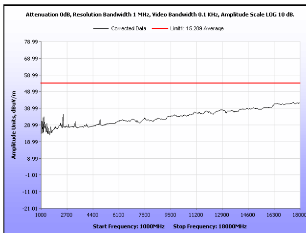
Plot 21. Radiated Spurious Emissions, Mid Channel, 802.11g, 1 GHz – 18 GHz, Average
