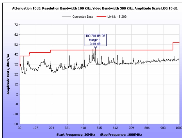
Plot 25. Radiated Spurious Emissions, Low Channel, 802.11n 20 MHz, 30 MHz – 1 GHz
