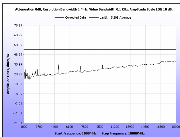
Plot 12. Radiated Spurious Emissions, Mid Channel, 802.11b, 1 GHz – 18 GHz, Average
