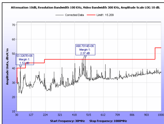
Plot 37. Radiated Spurious Emissions, Mid Channel, 802.11n 40 MHz, 30 MHz – 1 GHz
