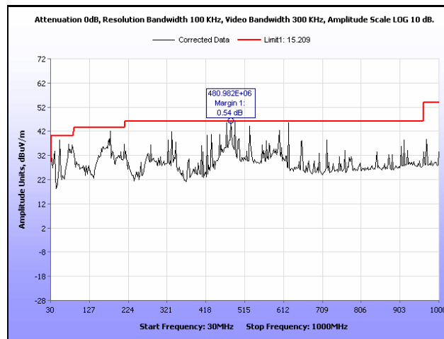
Plot 5. Radiated Spurious Emissions, Low Channel, 802.11b, 30 MHz – 1 GHz
