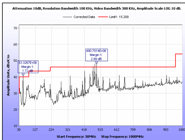
Plot 40. Radiated Spurious Emissions, High Channel, 802.11n 40 MHz, 30 MHz – 1 GHz
