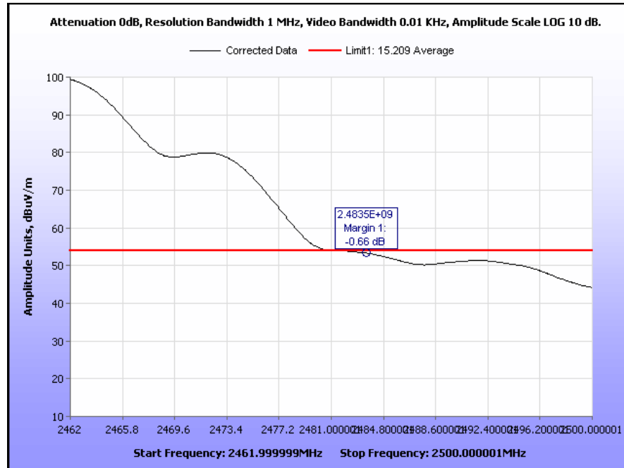
Plot 45. Radiated Restricted Band Edge, 802.11b, High Channel, Average
