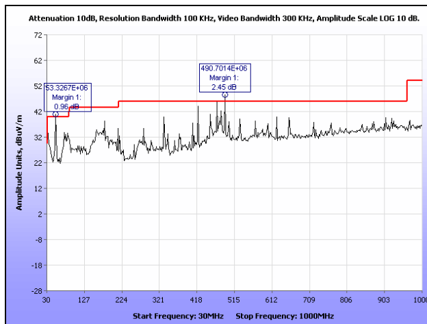
Plot 34. Radiated Spurious Emissions, Low Channel, 802.11n 40 MHz, 30 MHz – 1 GHz
