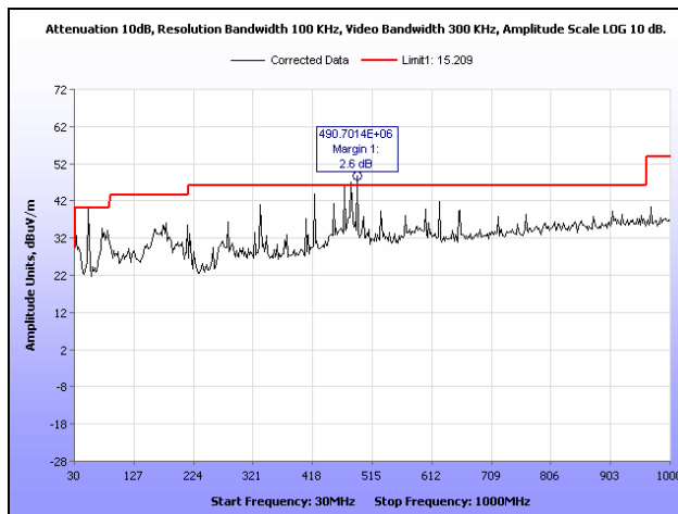
Plot 16. Radiated Spurious Emissions, Low Channel, 802.11g, 30 MHz – 1 GHz
