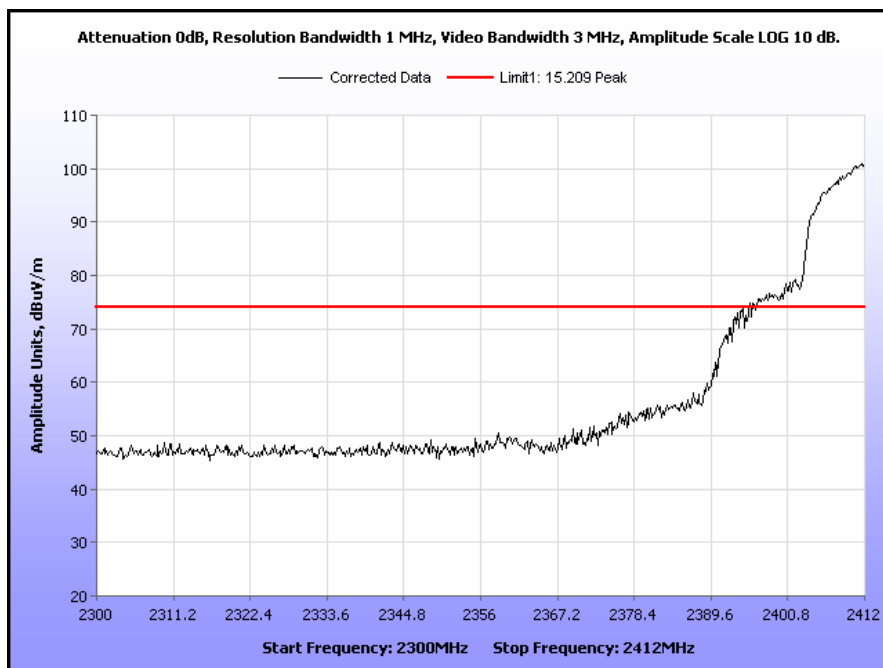
Plot 44. Radiated Restricted Band Edge, 802.11b, Low Channel, Peak
