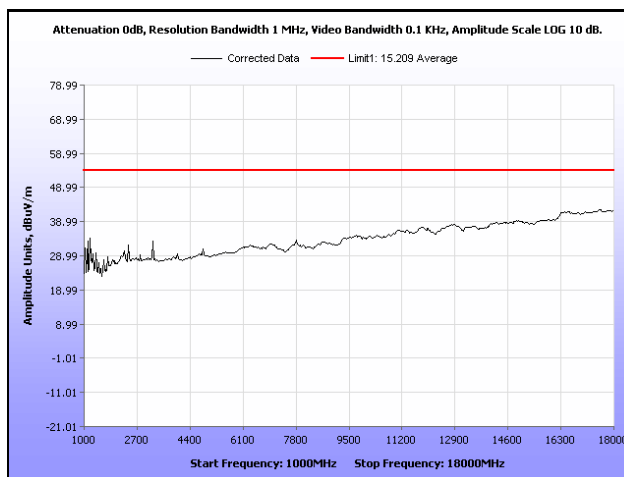
Plot 18. Radiated Spurious Emissions, Low Channel, 802.11g, 1 GHz – 18 GHz, Average
