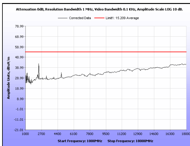
Plot 9. Radiated Spurious Emissions, Low Channel, 802.11b, 1 GHz – 18 GHz, Average
