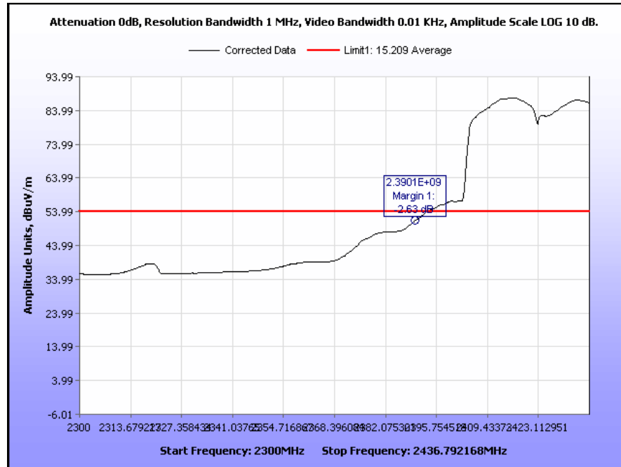
Plot 55. Radiated Restricted Band Edge, 802.11n 40 MHz, Low Channel, Average
