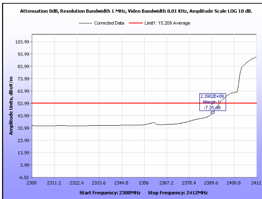
Plot 43. Radiated Restricted Band Edge, 802.11b, Low Channel, Average
