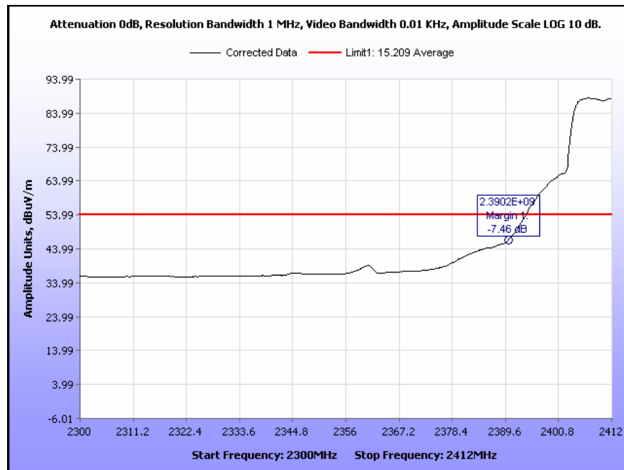
Plot 47. Radiated Restricted Band Edge, 802.11g, Low Channel, Average
