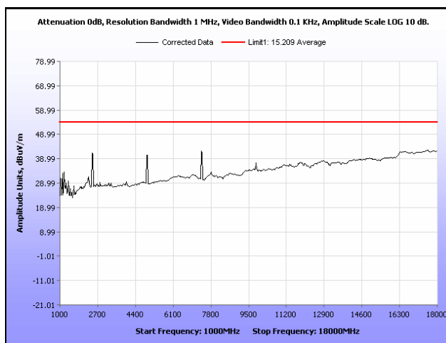
Plot 15. Radiated Spurious Emissions, High Channel, 802.11b, 1 GHz – 18 GHz, Average
