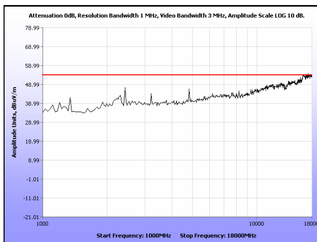
Plot 35. Radiated Spurious Emissions, Low Channel, 802.11n 40 MHz, 1 GHz – 18 GHz, Peak
