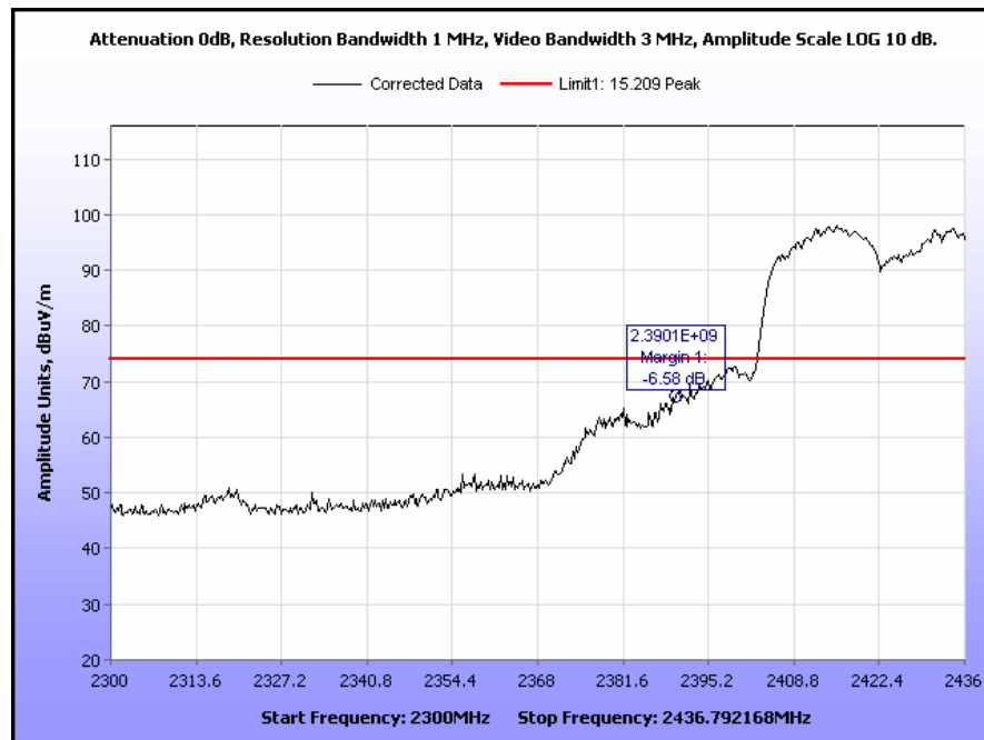
Plot 56. Radiated Restricted Band Edge, 802.11n 40 MHz, Low Channel, Peak
