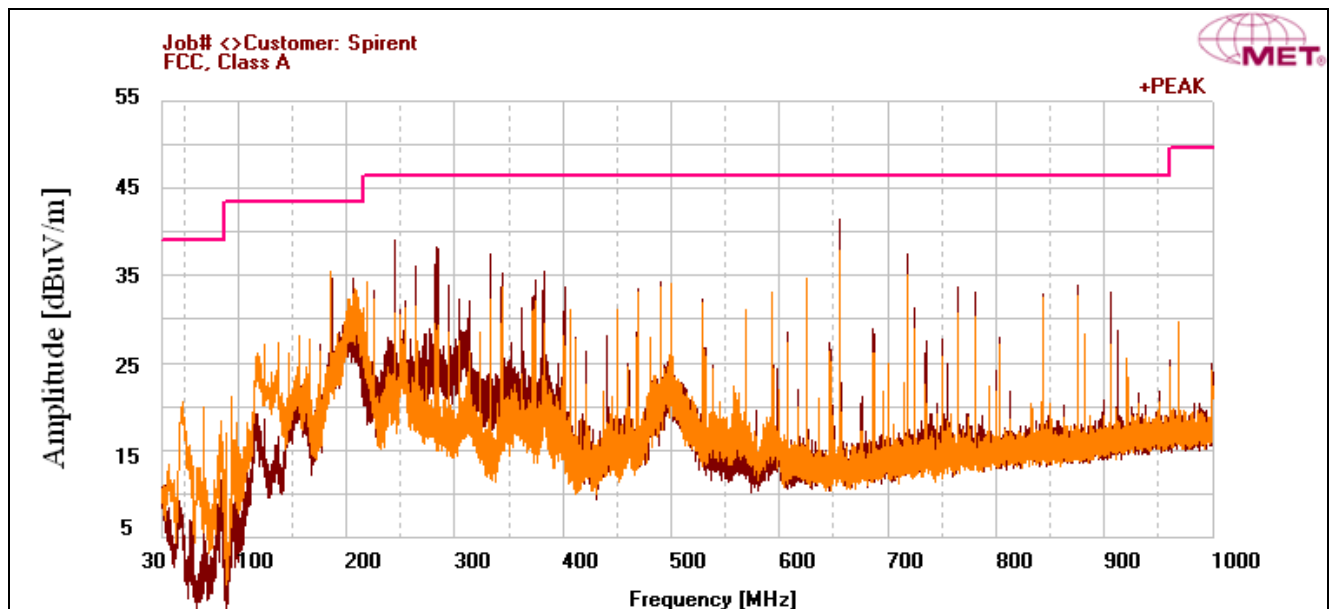
Plot 3. Radiated Emissions, 30 MHz - 1 GHz
