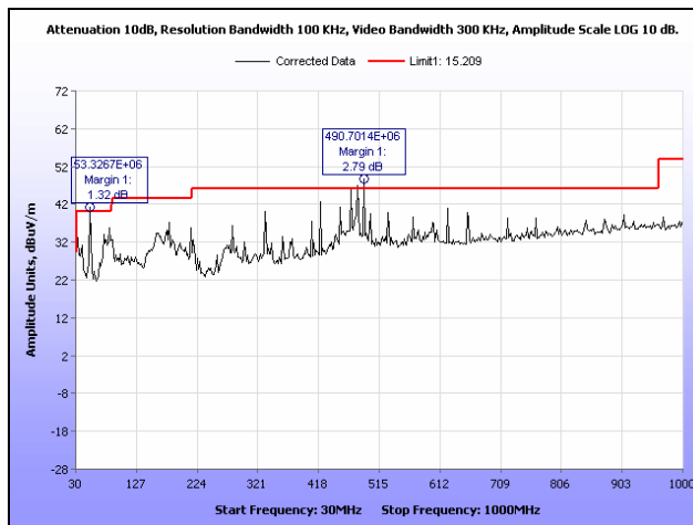
Plot 31. Radiated Spurious Emissions, High Channel, 802.11n 20 MHz, 30 MHz – 1 GHz
