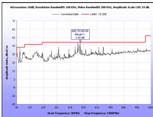
Plot 10. Radiated Spurious Emissions, Mid Channel, 802.11b, 30 MHz – 1 GHz
