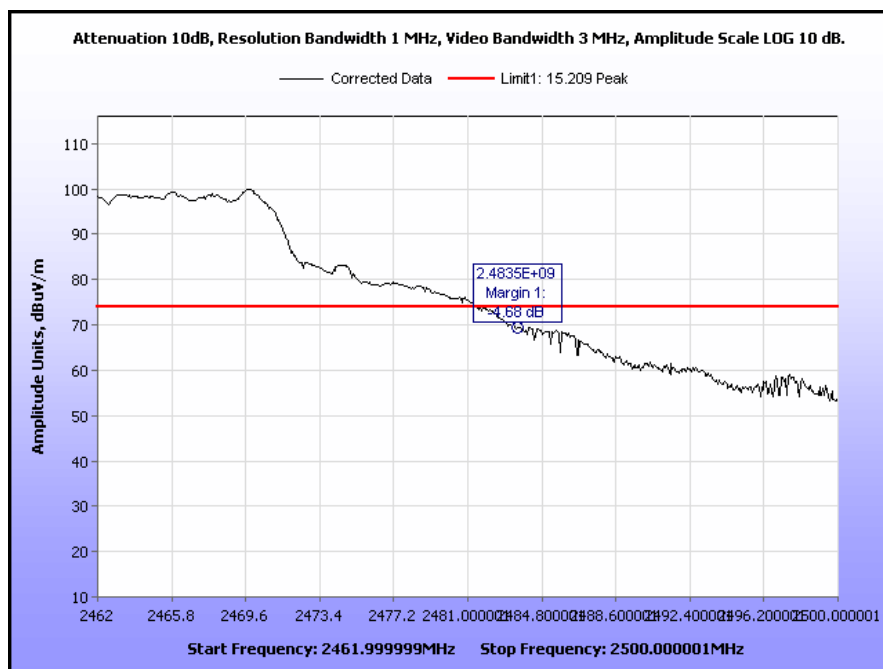
Plot 54. Radiated Restricted Band Edge, 802.11n 20 MHz, High Channel, Peak
