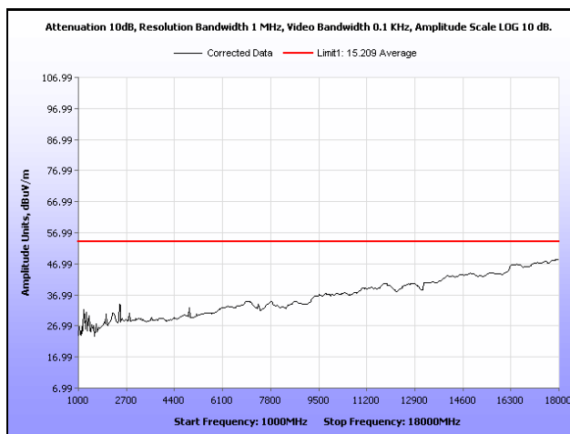
Plot 42. Radiated Spurious Emissions, High Channel, 802.11n 40 MHz, 1 GHz – 18 GHz, Average
