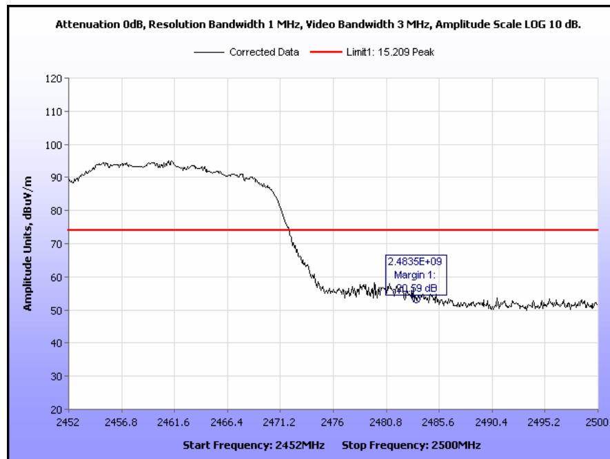
Plot 58. Radiated Restricted Band Edge, 802.11n 40 MHz, High Channel, Peak
