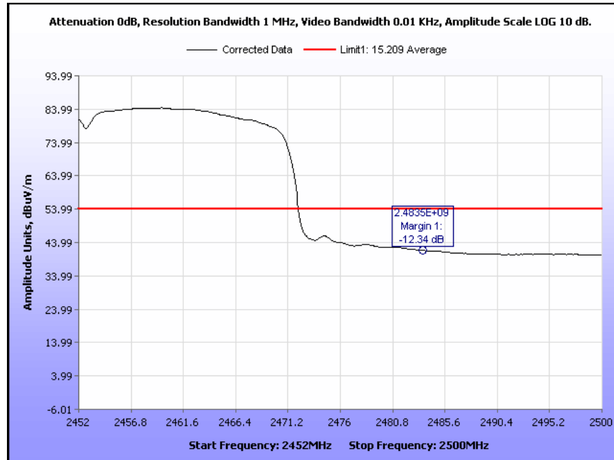
Plot 57. Radiated Restricted Band Edge, 802.11n 40 MHz, High Channel, Average
