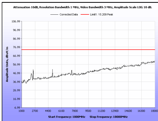
Plot 32. Radiated Spurious Emissions, High Channel, 802.11n 20 MHz, 1 GHz – 18 GHz, Peak
