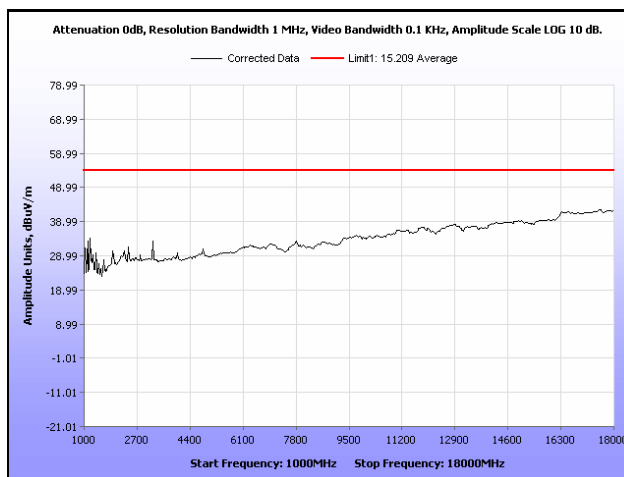
Plot 36. Radiated Spurious Emissions, Low Channel, 802.11n 40 MHz, 1 GHz – 18 GHz, Average
