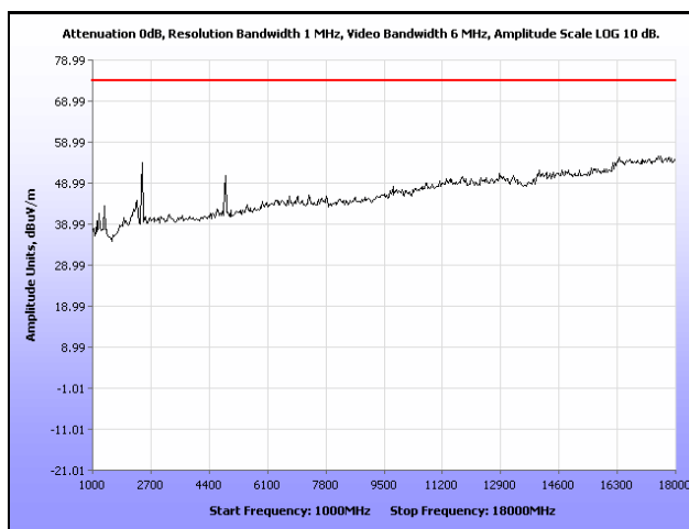
Plot 20. Radiated Spurious Emissions, Mid Channel, 802.11g, 1 GHz – 18 GHz, Peak
