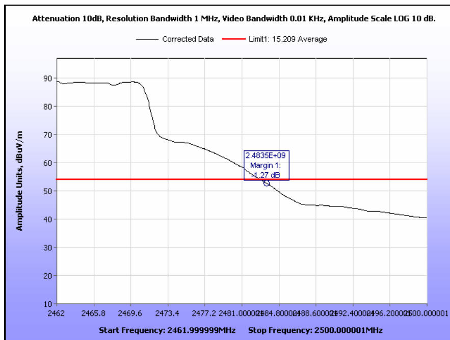
Plot 53. Radiated Restricted Band Edge, 802.11n 20 MHz, High Channel, Average
