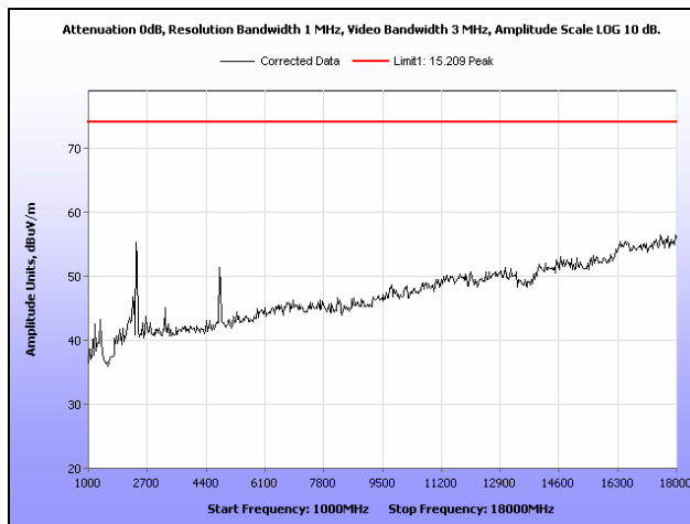
Plot 8. Radiated Spurious Emissions, Low Channel, 802.11b, 1 GHz – 18 GHz, Peak
