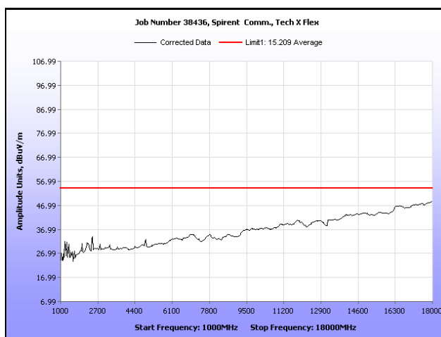
Plot 30. Radiated Spurious Emissions, Mid Channel, 802.11n 20 MHz, 1 GHz – 18 GHz, Average
