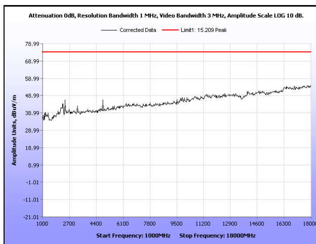
Plot 17. Radiated Spurious Emissions, Low Channel, 802.11g, 1 GHz – 18 GHz, Peak
