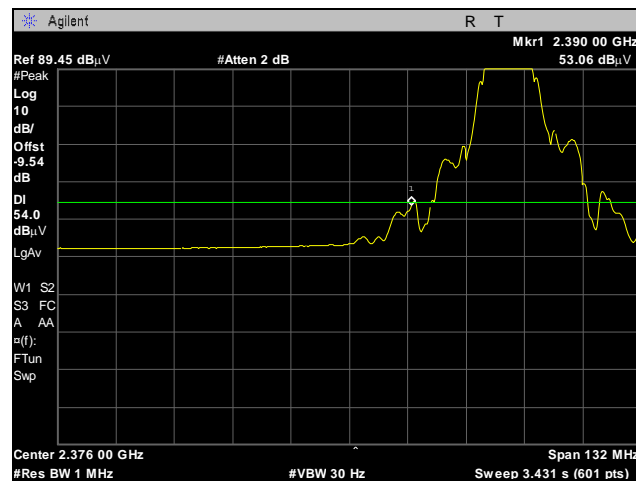
Plot 35. Radiated Band Edge, 802.11b, Average, Low Channel
