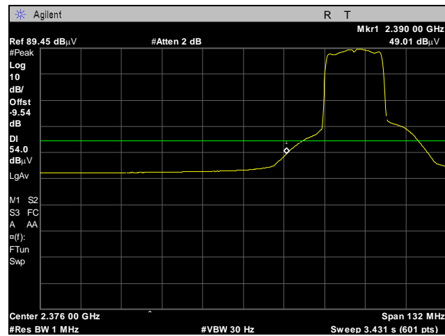
Plot 43. Radiated Band Edge, 802.11n, Average, Low Channel
