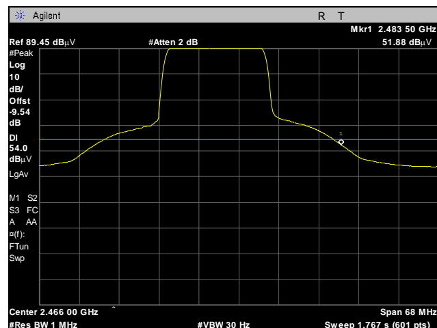
Plot 41. Radiated Band Edge, 802.11g, Average, High Channel
