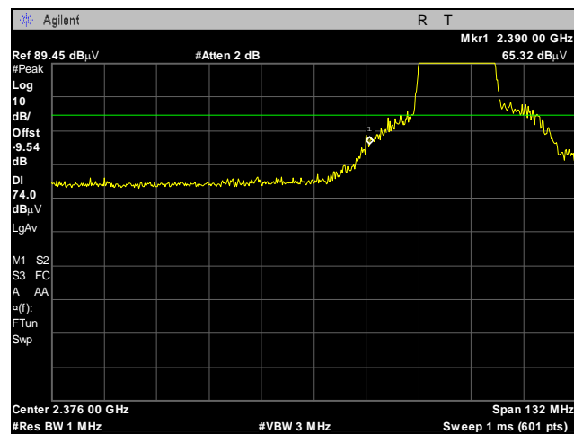
Plot 44. Radiated Band Edge, 802.11n, Peak, Low Channel
