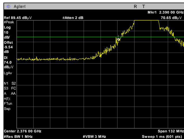
Plot 40. Radiated Band Edge, 802.11g, Peak, Low Channel
