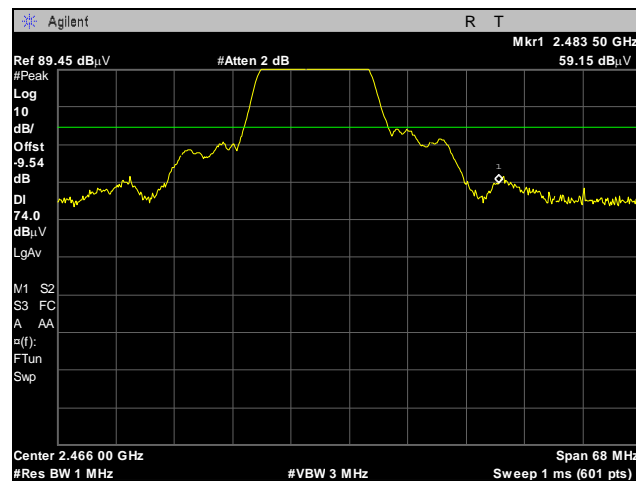
Plot 38. Radiated Band Edge, 802.11b, Peak, High Channel
