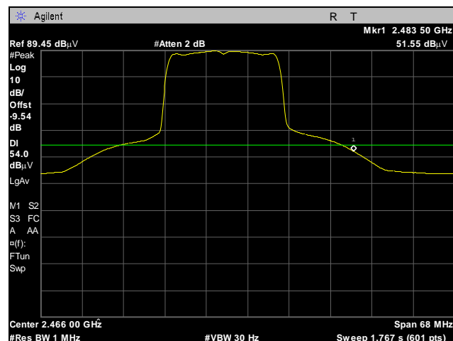
Plot 45. Radiated Band Edge, 802.11n, Average, High Channel
