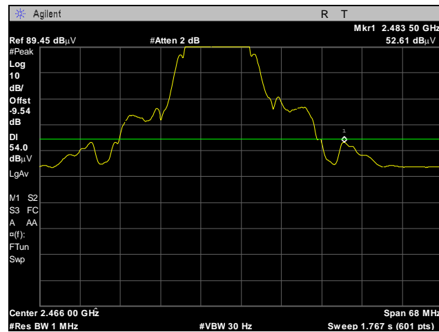
Plot 37. Radiated Band Edge, 802.11b, Average, High Channel
