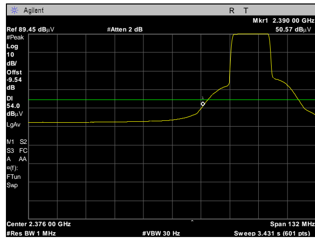
Plot 39. Radiated Band Edge, 802.11g, Average, Low Channel
