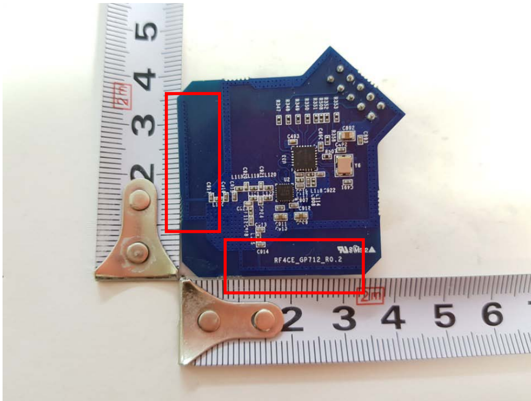
ZIGBEE_Antenna
