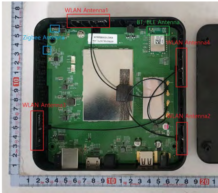
[WLAN_Antenna1]
