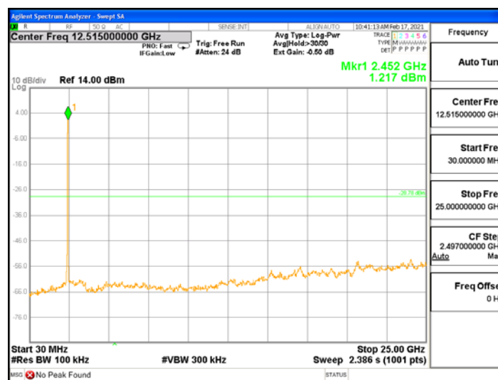
ANT4, 802.11n_HT40
