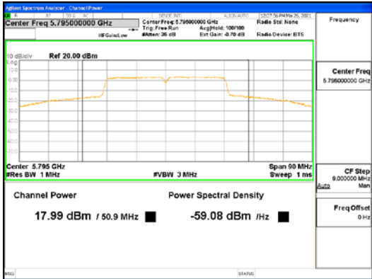
ANT3_802.11ac_VHT40_UNII 3
