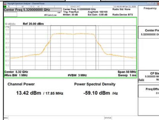
CDD Mode_ANT4_802.11a_UNII 2A
