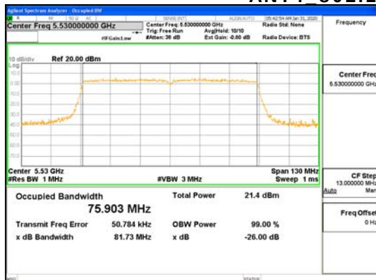
ANT4 802.11ac_VHT80_UNII 2C
