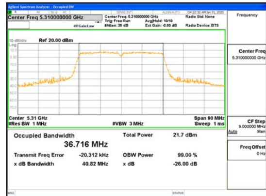
ANT4_802.11ac_VHT40_UNII 2A
