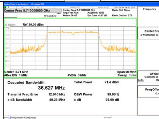
ANT3_802.11n_HT40_UNII 2C
