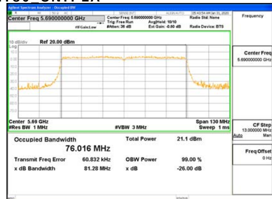
ANT4 802.11ac_VHT80_UNII 2C
