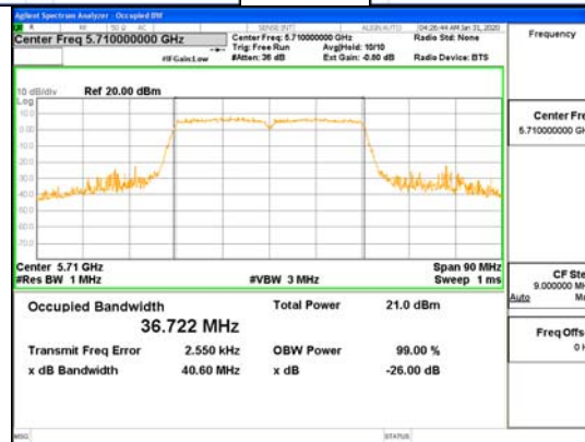
ANT4_802.11ac_VHT40_UNII 2C
