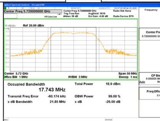
ANT4_802.11a_UNII 2C
