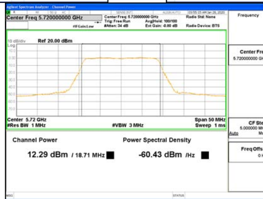
CDD Mode_ANT4_802.11ac_VHT20_UNII 2C
