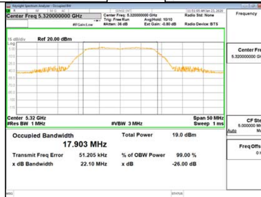
ANT3_802.11a_UNII 2A
