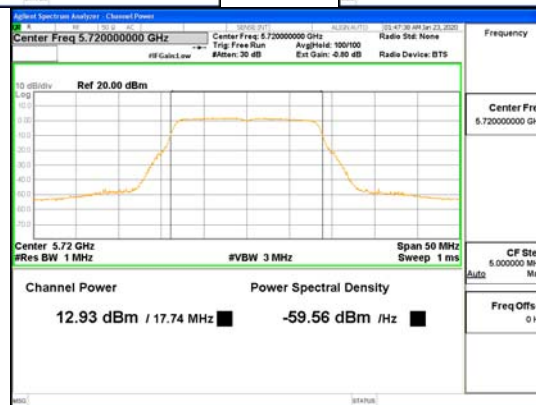
CDD Mode_ANT4_802.11a_UNII 2C
