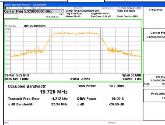
ANT4_802.11n_HT20_UNII 2A
