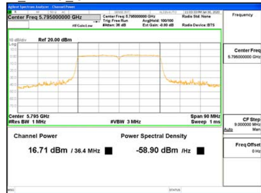
SDM Mode ANT3_802.11n_HT40_UNII-3
