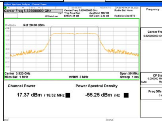
SDM Mode_ANT4_802.11ac_VHT20_UNII-3
