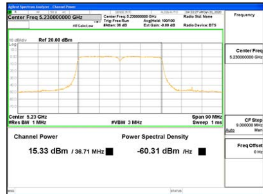
SDM Mode ANT3 802.11ac VHT40 UNII-1
