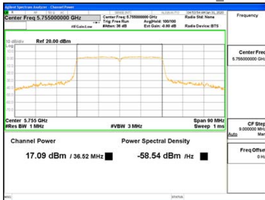
SDM Mode ANT2 802.11ac VHT40 UNII-3
