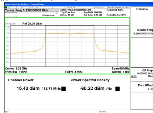
SDM Mode ANT4 802.11ac VHT40 UNII-1
