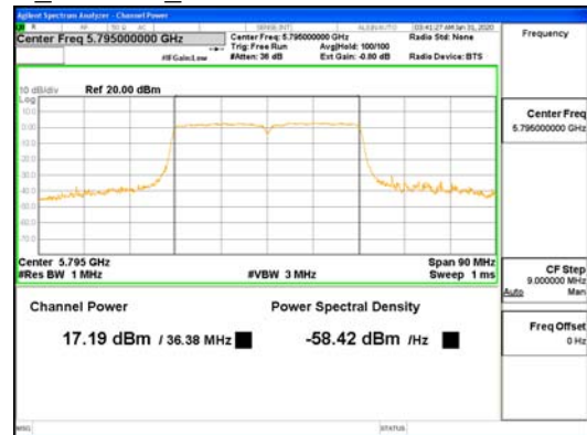
CDD Mode ANT4 802.11ac VHT40 UNII-3
