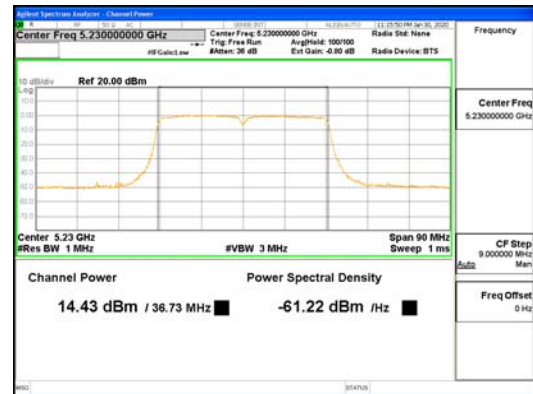
SDM Mode ANT1_802.11n_HT40_UNII-1
