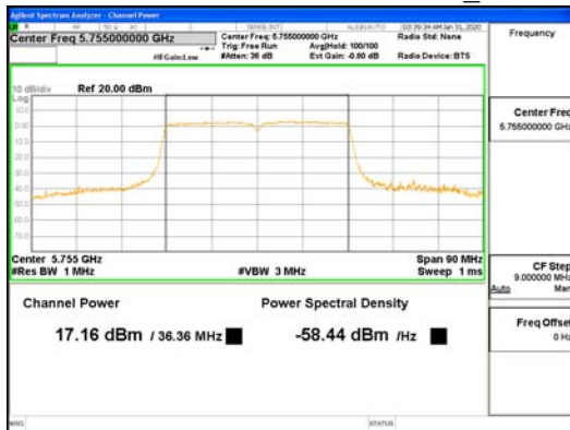
CDD Mode ANT4 802.11ac VHT40 UNII-3
