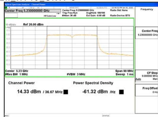
SDM Mode ANT4_802.11n_HT40_UNII-1
