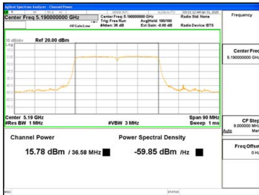
CDD Mode ANT3 802.11ac VHT40 UNII-1
