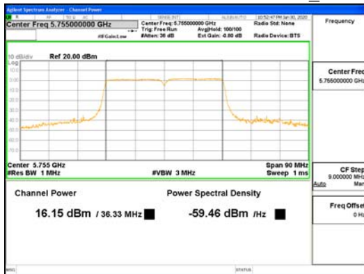
SDM Mode ANT4_802.11n_HT40_UNII-3
