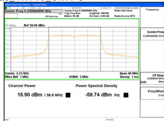
CDD Mode ANT2 802.11ac VHT40 UNII-1
