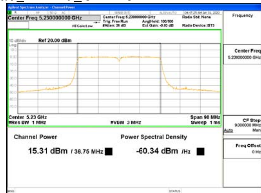
SDM Mode ANT2 802.11ac VHT40 UNII-1
