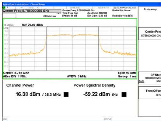
SDM Mode ANT3_802.11n_HT40_UNII-3
