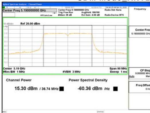
SDM Mode ANT2 802.11ac VHT40 UNII-1
