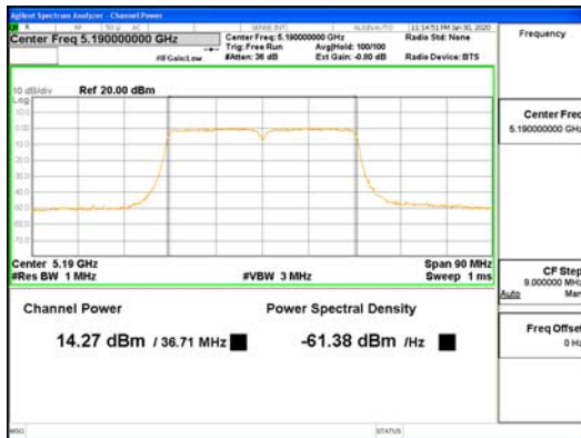
SDM Mode ANT1_802.11n_HT40_UNII-1
