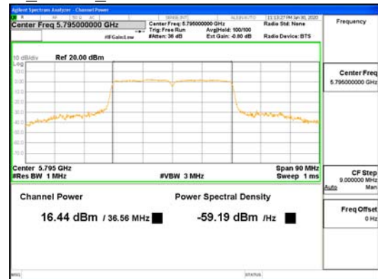
SDM Mode ANT2_802.11n_HT40_UNII-3
