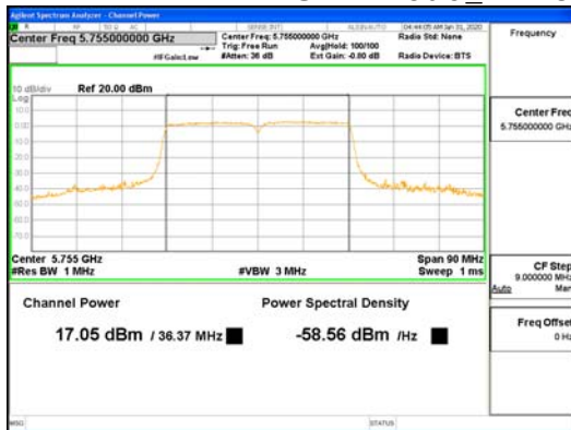
SDM Mode ANT3 802.11ac VHT40 UNII-3
