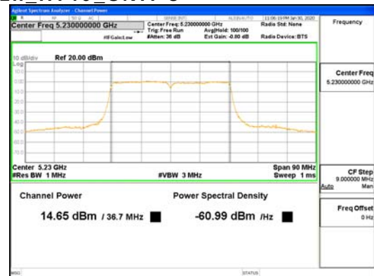
SDM Mode ANT2_802.11n_HT40_UNII-1
