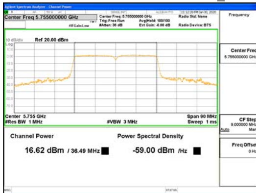
SDM Mode ANT2_802.11n_HT40_UNII-3
