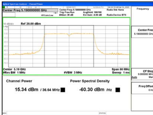
SDM Mode ANT3 802.11ac VHT40 UNII-1
