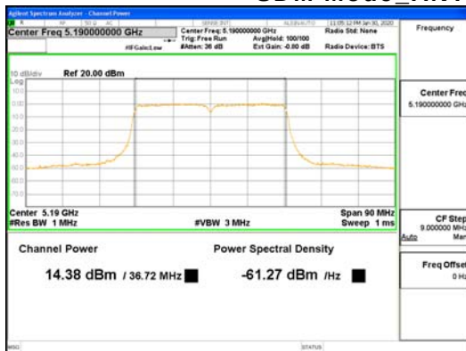
SDM Mode ANT2_802.11n_HT40_UNII-1
