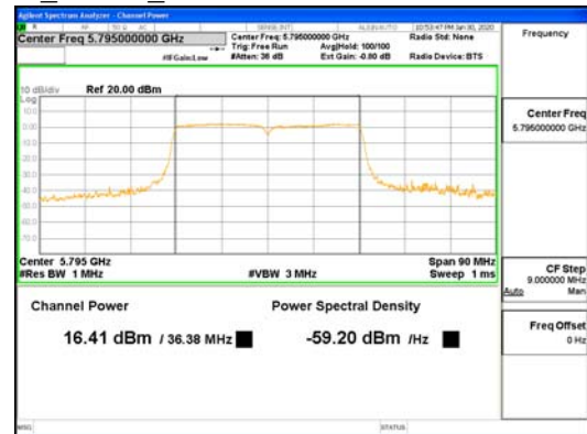
SDM Mode ANT4_802.11n_HT40_UNII-3
