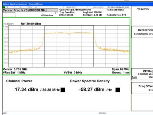
CDD Mode ANT3 802.11ac VHT40 UNII-3
