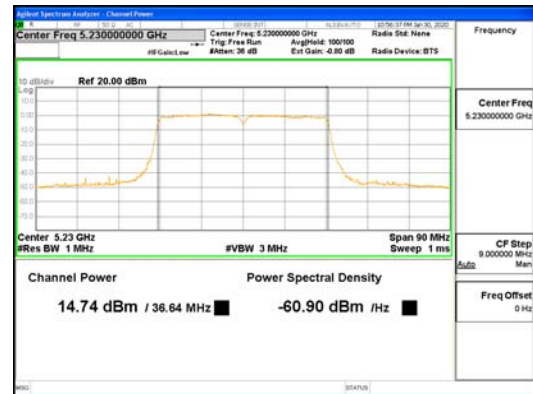
SDM Mode ANT3_802.11n_HT40_UNII-1
