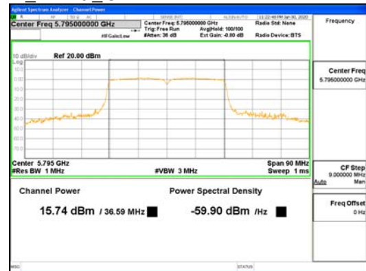
SDM Mode ANT1_802.11n_HT40_UNII-3
