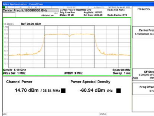
SDM Mode ANT3_802.11n_HT40_UNII-1
