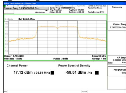
SDM Mode ANT2 802.11ac VHT40 UNII-3
