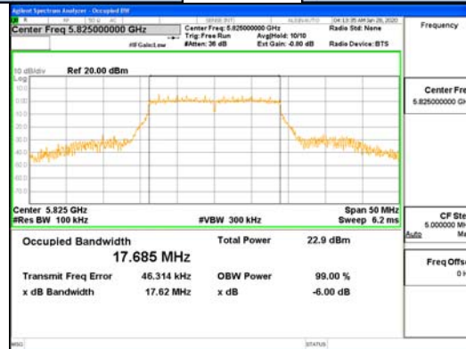
ANT4_802.11ac_VHT20
