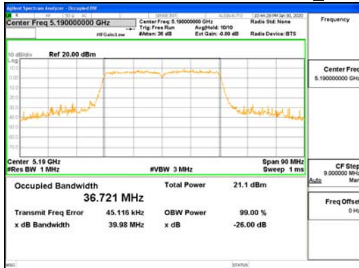
ANT4_802.11n_HT40_UNII-1
