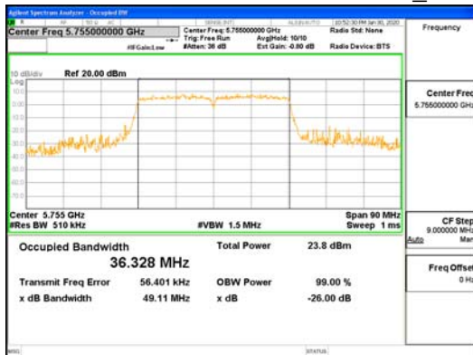
ANT4_802.11n_HT40_UNII-3
