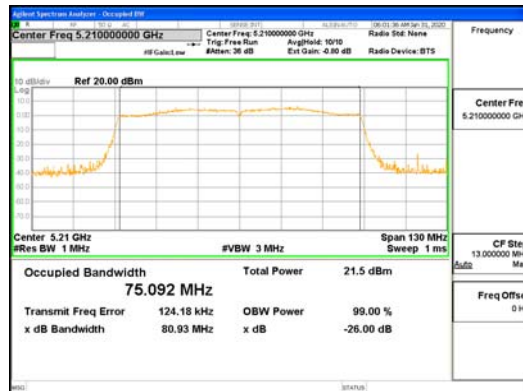
ANT1_802.11ac_VHT80_UNII-1
