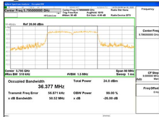
ANT4_802.11n_HT40_UNII-3
