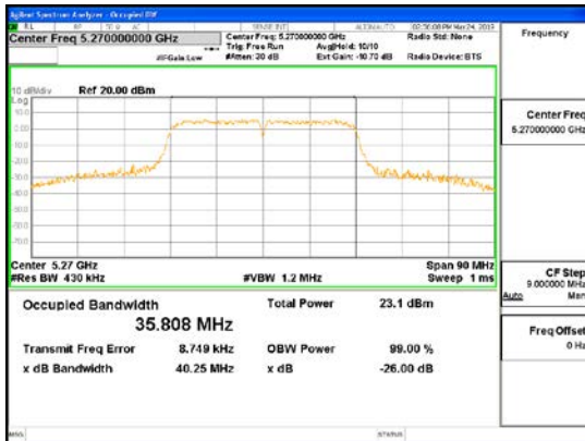
ANT2_802.11n_HT40_UNII 2A
