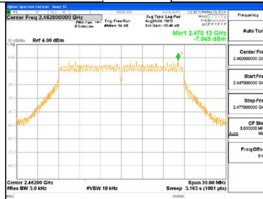
SDM Mode_802.11n_HT20_ANT2
