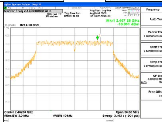
CDD Mode_802.11n_HT20_ANT1
