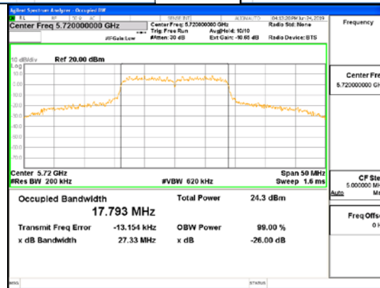
ANT2_802.11n_HT20_UNII 2C
