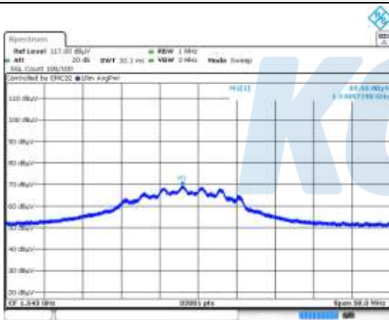
Average data (1 540.97 MHz)
