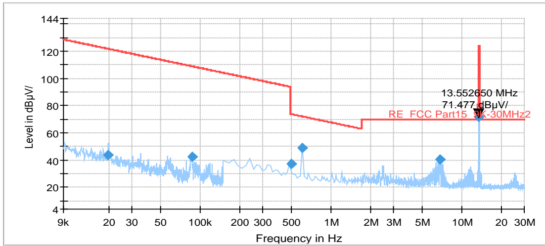
Radiates Emission from 9kHz to 30MHz
