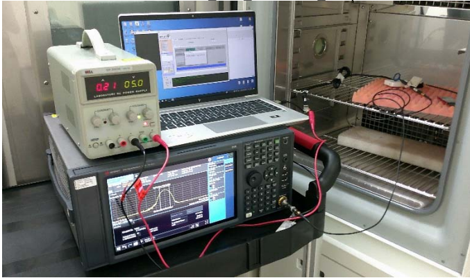
P15.225+RSS210 NFC Radiated Setup
