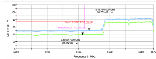
802.11ac VHT80-Channel 106: Peak + Average
