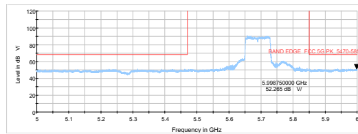
802.11ac VHT80-Channel 138: Peak
