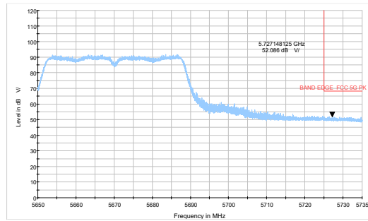
802.11n HT40-Channel 134: Peak
