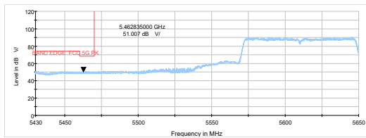
802.11ac VHT80-Channel 122: Peak
