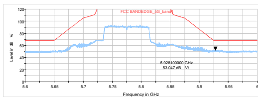
802.11ac VHT80- Channel 155: Peak
