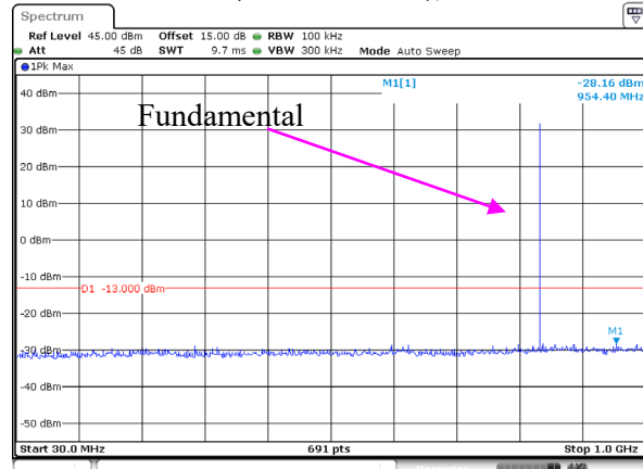
30 MHz – 1GHz (EGPRS Mode), Middle channel
