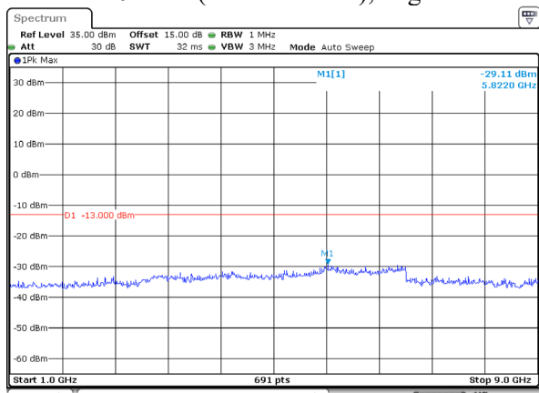
1 GHz – 9 GHz (EGPRS Mode), High channel
