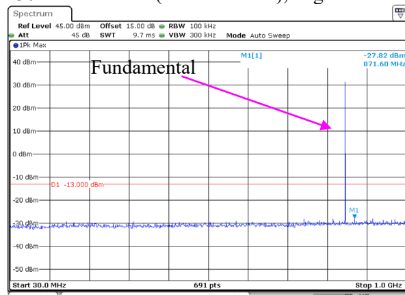
30 MHz – 1GHz (EGPRS Mode), High channel
