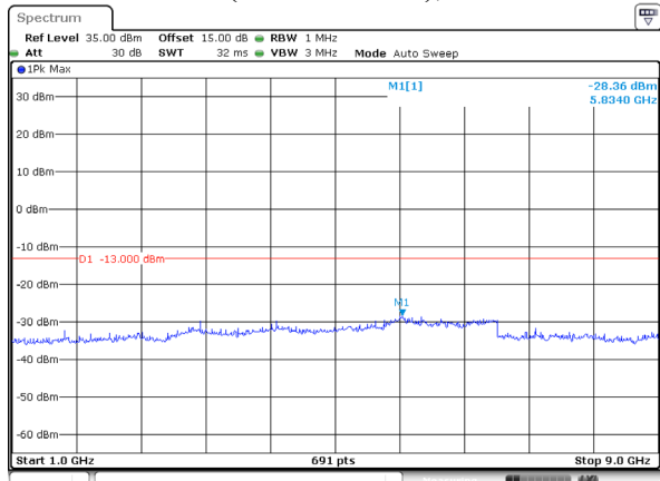
1 GHz – 9 GHz (EGPRS Mode), Middle channel
