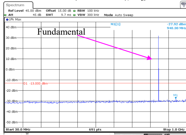
30 MHz – 1GHz (GPRS Mode), High channel
