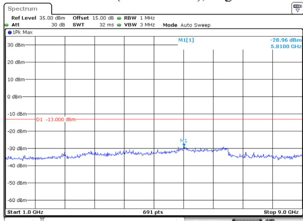
1 GHz – 9 GHz (GPRS Mode), High channel
