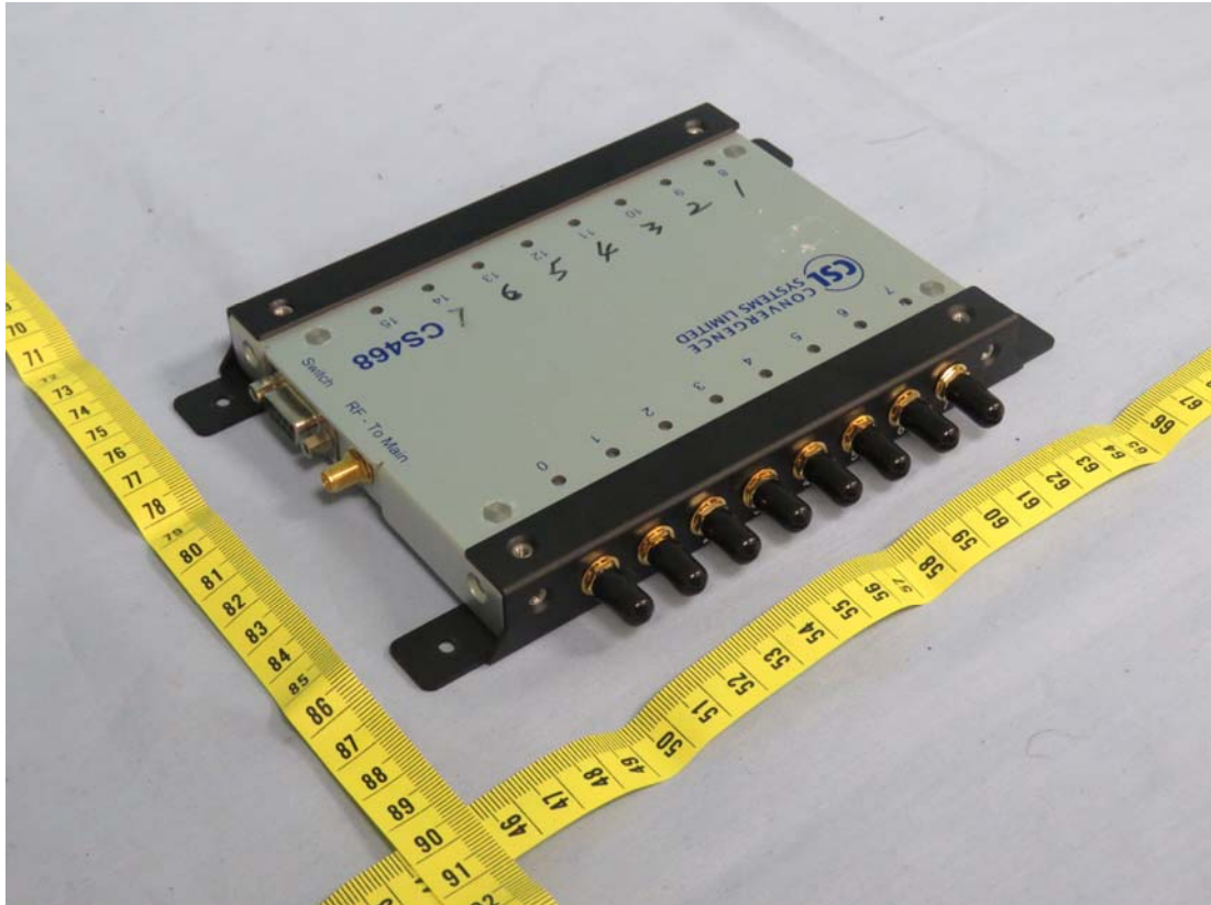
Figure 23 Internal View
