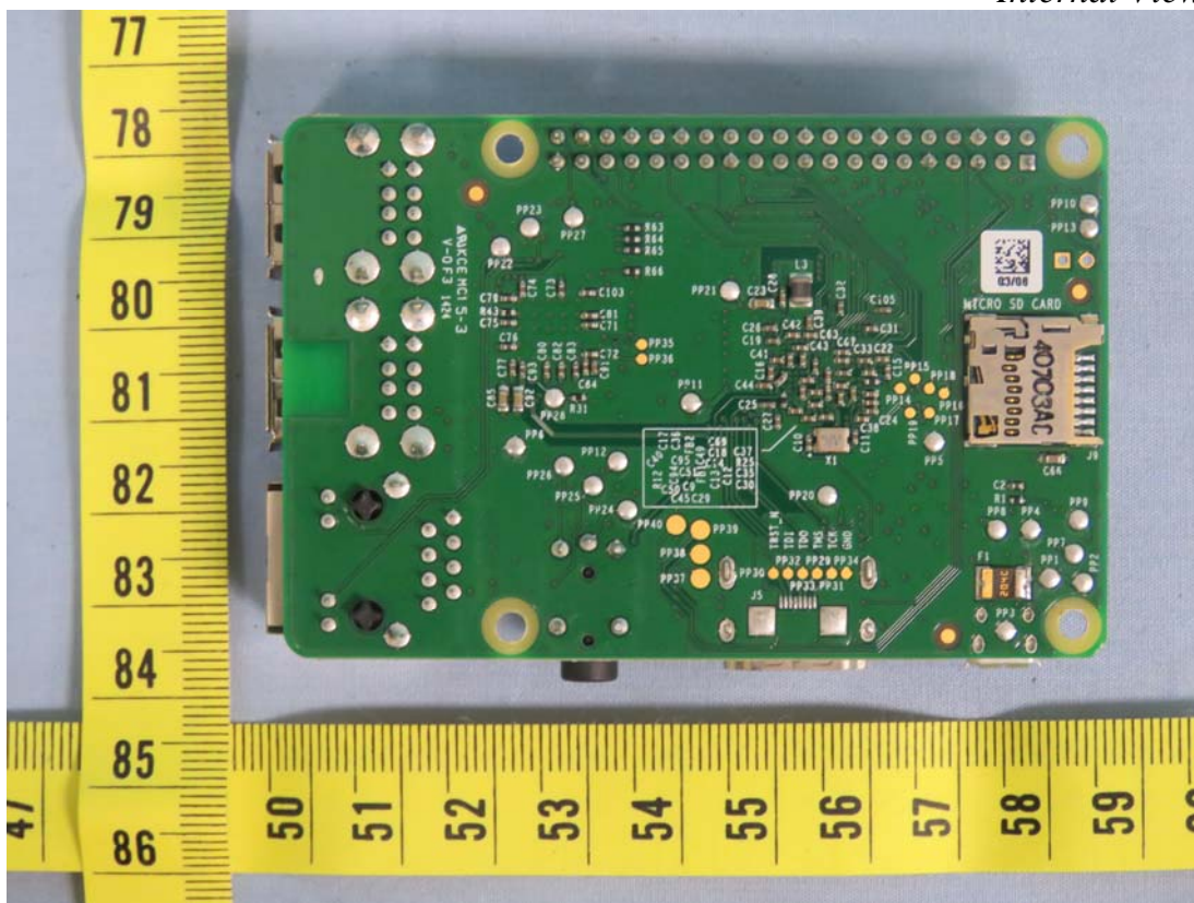
Figure 12 Internal View
