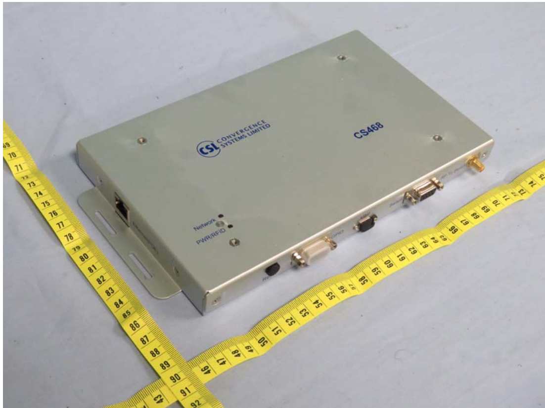
Figure 19 Internal View
