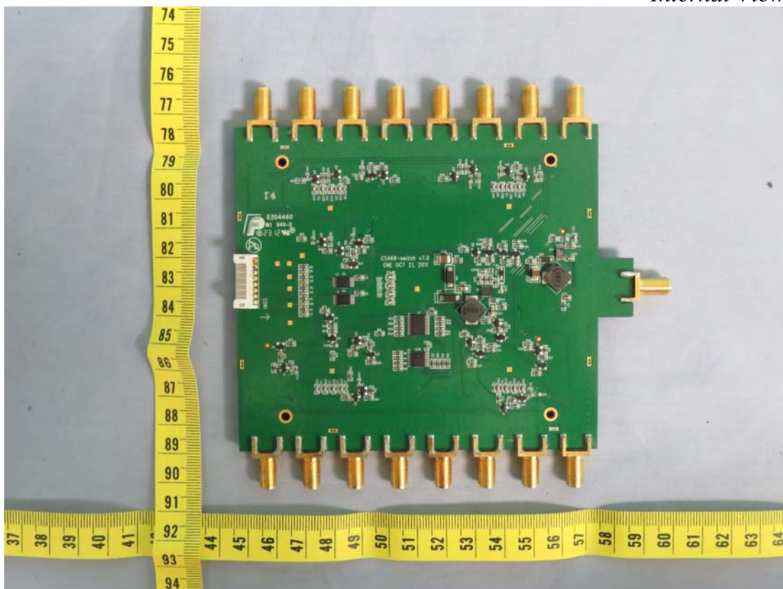
Figure 26 Internal View
