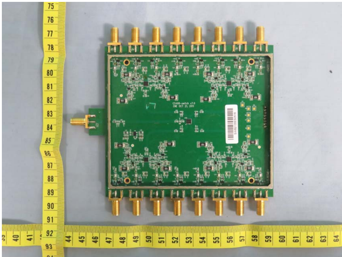
Figure 25 Internal View
