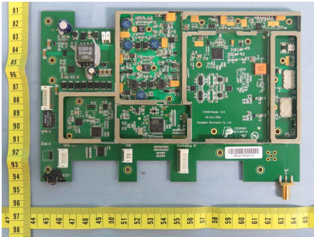
Figure 21 Internal View
