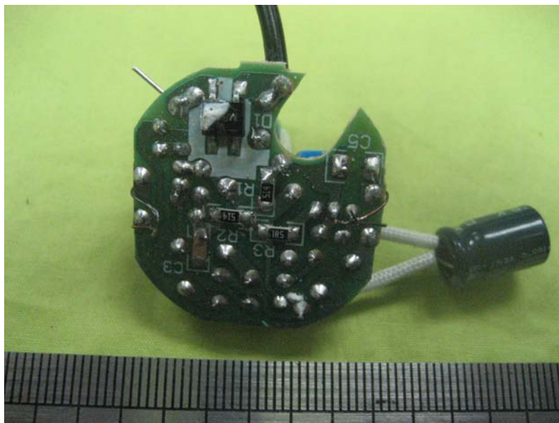
Bottom View of PCB (8W/ELX)
