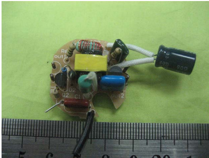
Top View of PCB (8W/ELX)
