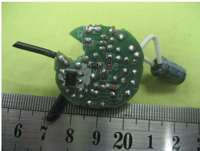
Bottom View of PCB (7W/ELX)
