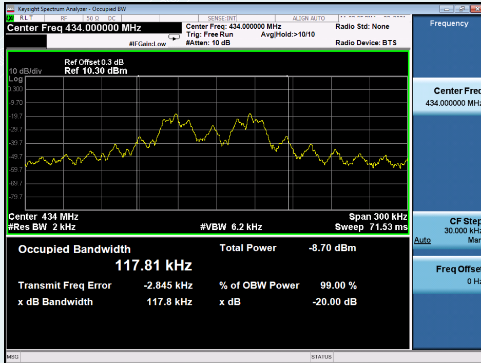
434MHz FSK
