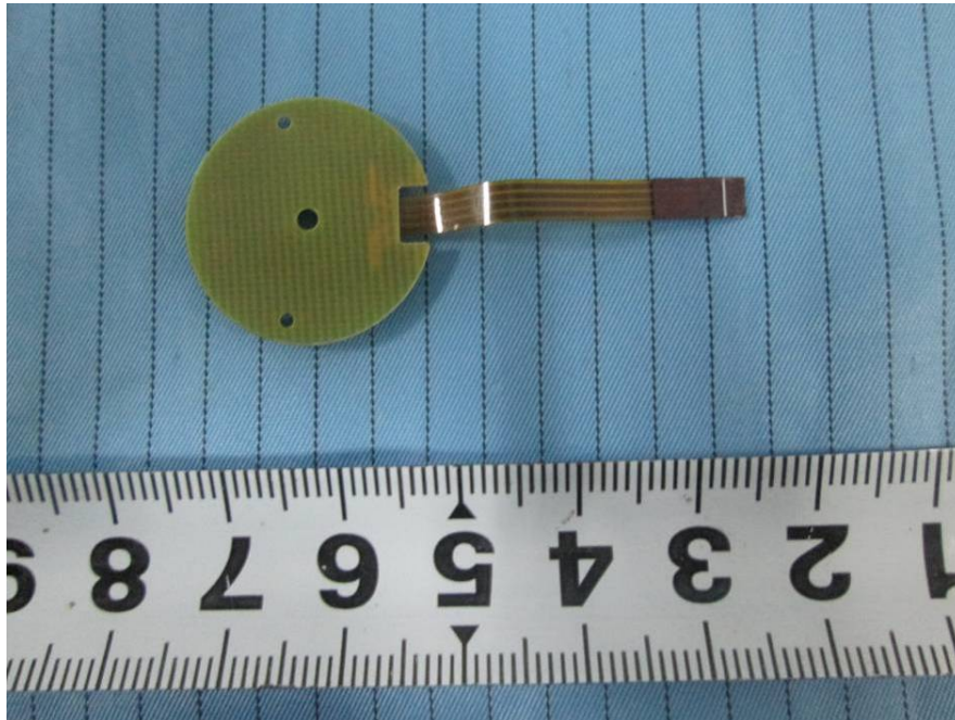
EUT –LED Board 2 Bottom View
