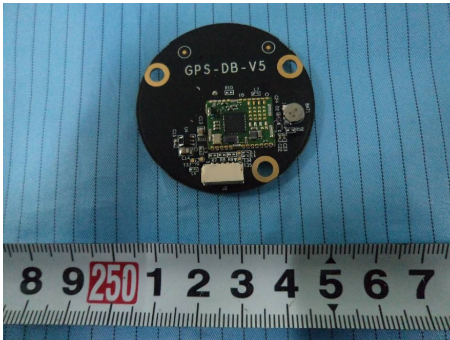
EUT –GPS Board Top Shielding Off View
