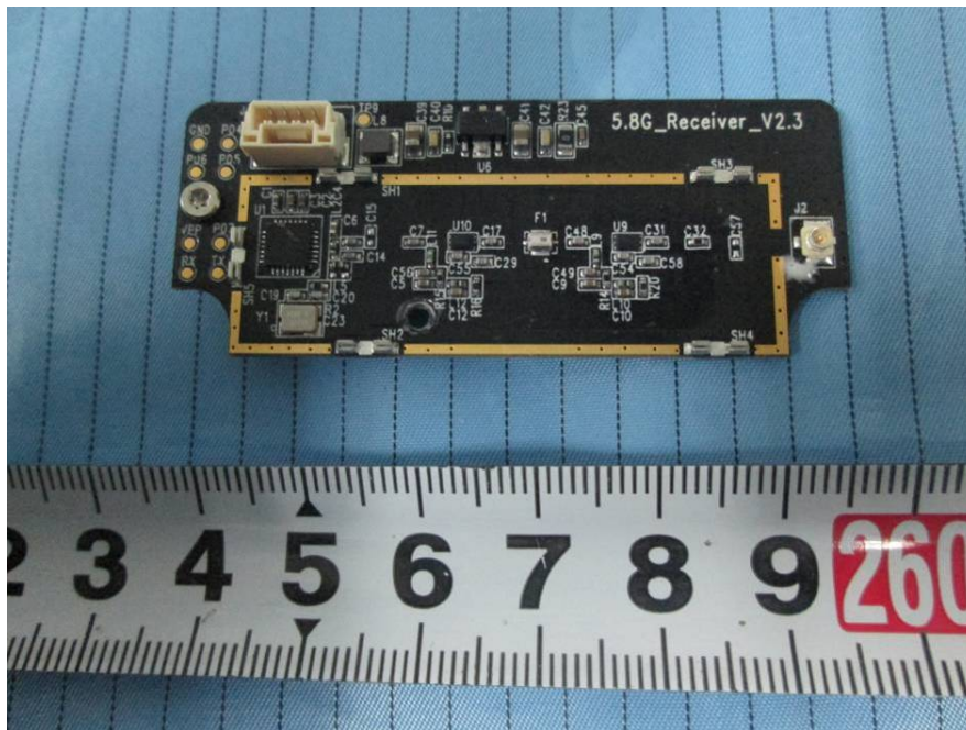
EUT – 5.8G_Receiver Board Top View
