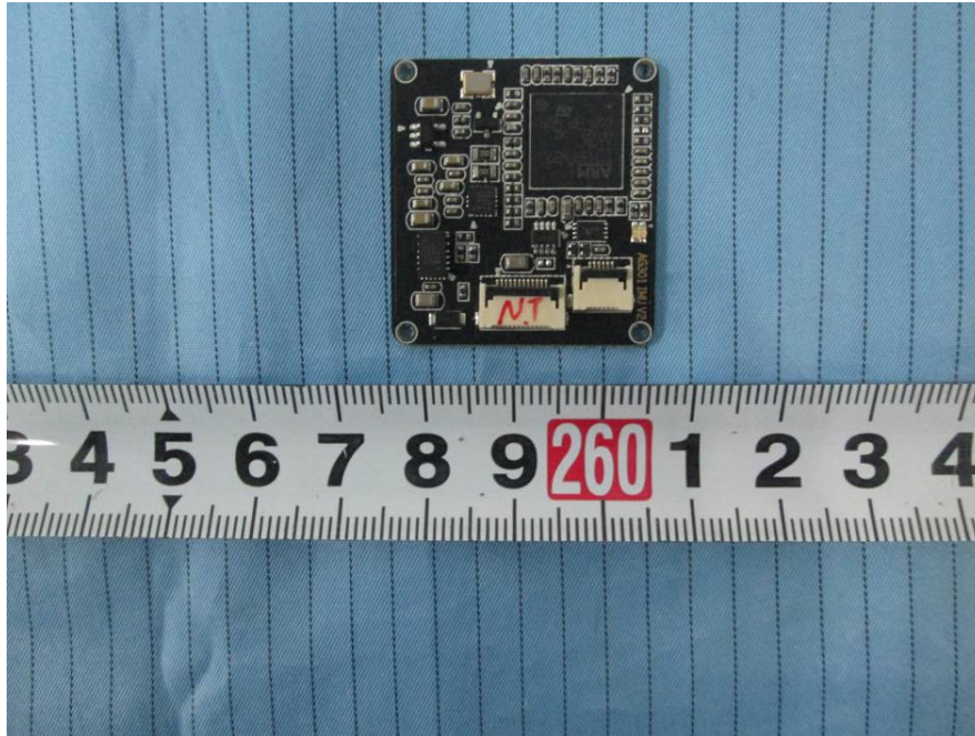
EUT – Camera Board 1 Top View
