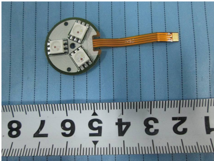
EUT –LED Board 3 Top View
