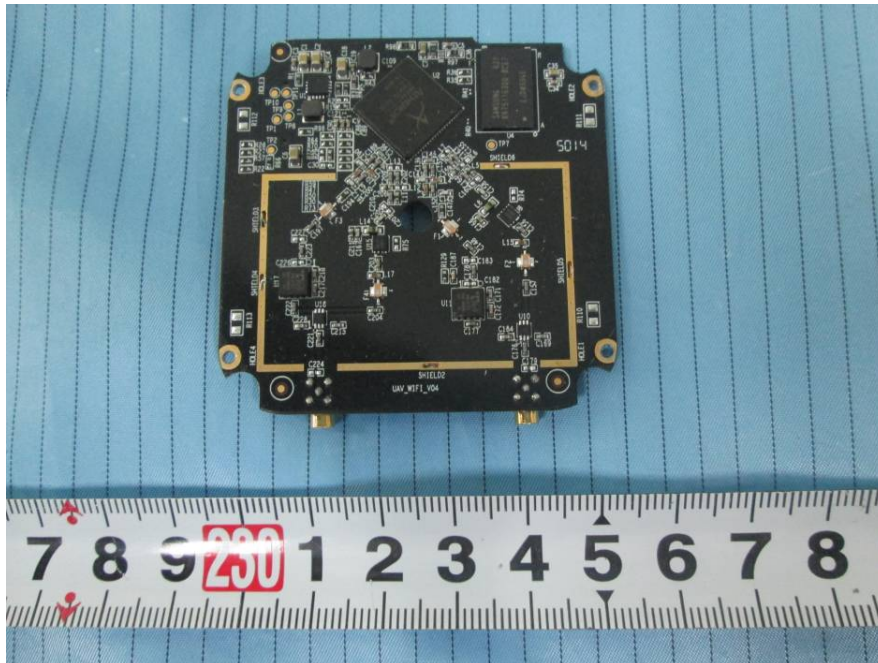
EUT – Wifi Board Top Shielding Off View
