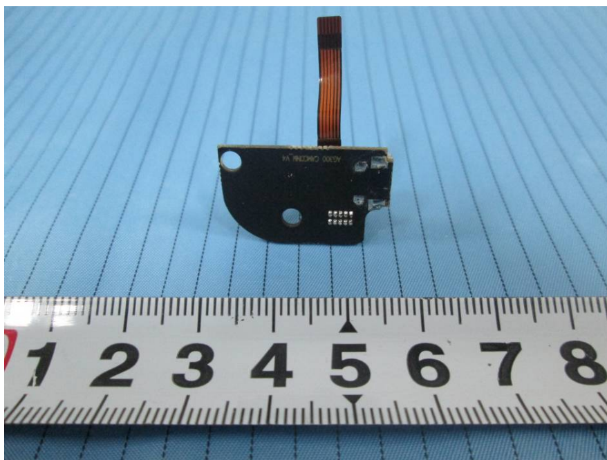
EUT – Camera USB Board 1 Bottom View
