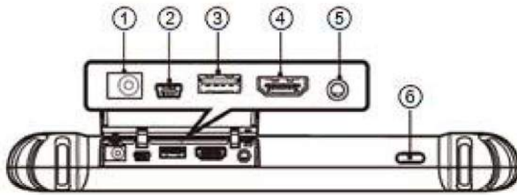
Figure 2-3 Tablet Top View
