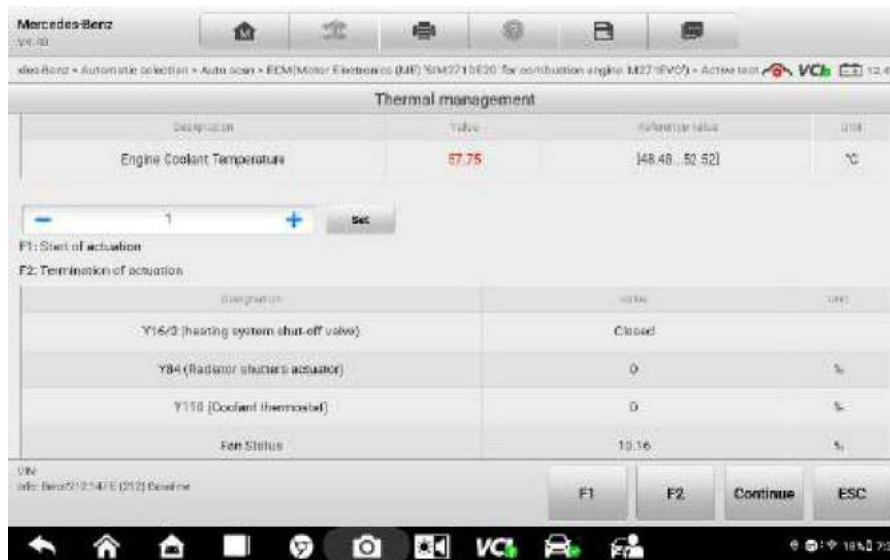
Figure 4-16 Sample Active Test Screen
