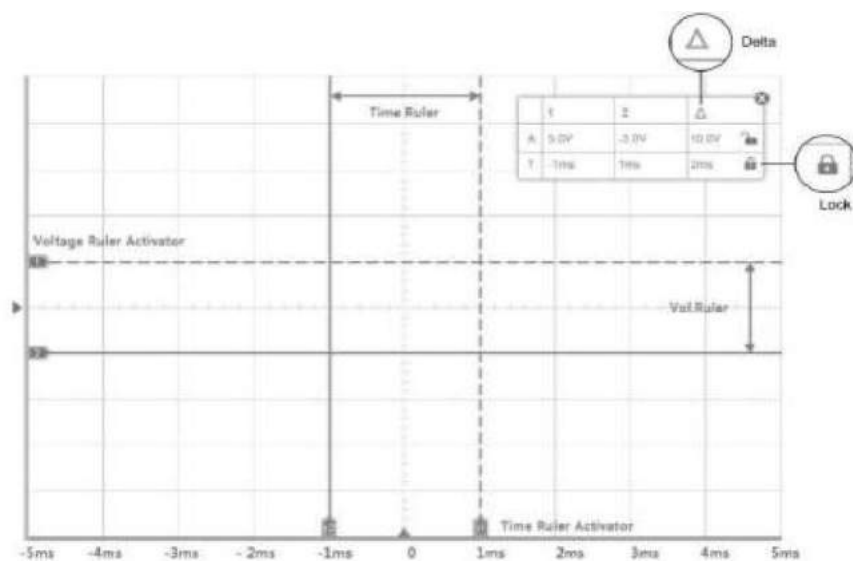
Figure 19-8 Measurement Rulers Display
