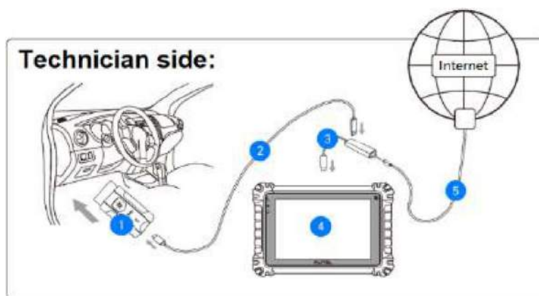
Figure 8-1 Sample connection diagram on Technician side
