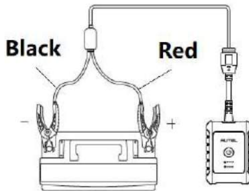
Figure 9-2 Connecting to a Battery
