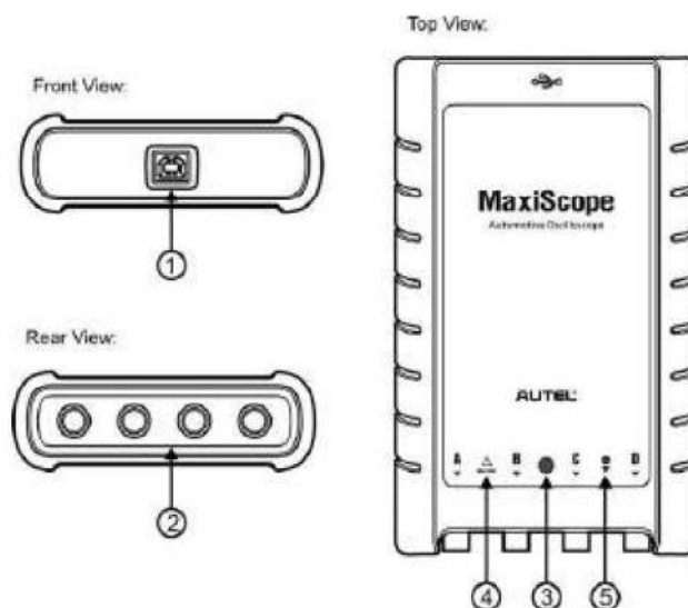
Figure 19-3 MaxiScope Front, Rear, and Top View
