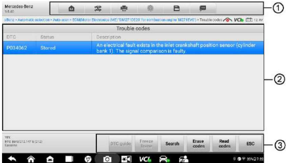
Figure 4-10 Sample Read Codes Screen
