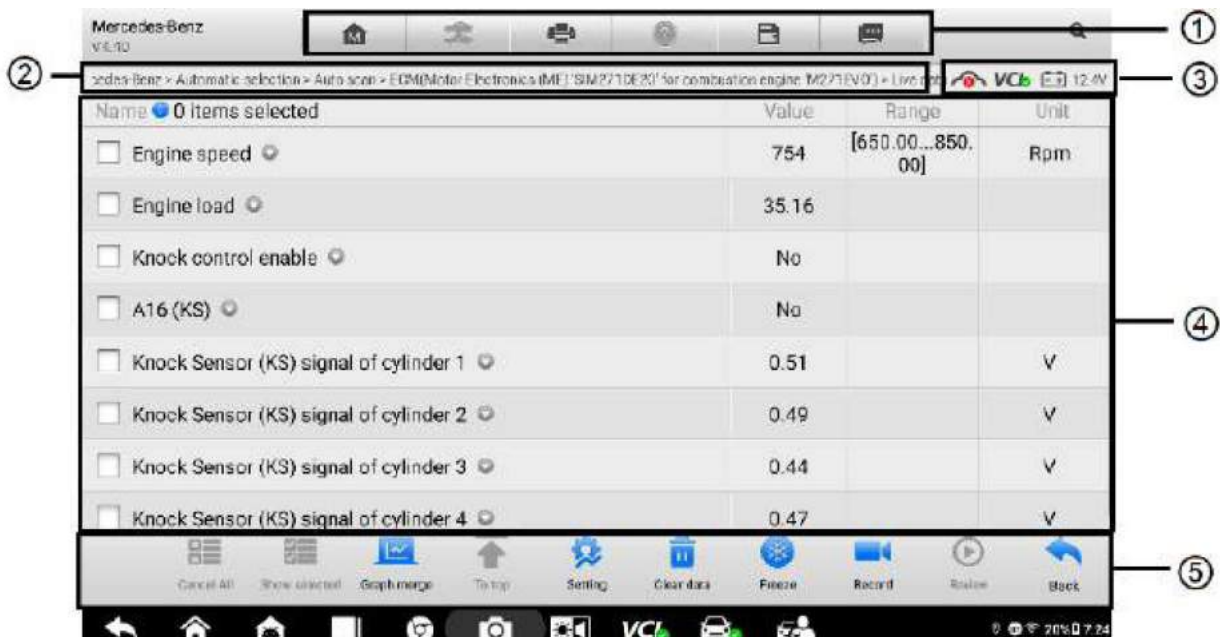
Figure 4-11 Sample Live Data Screen
