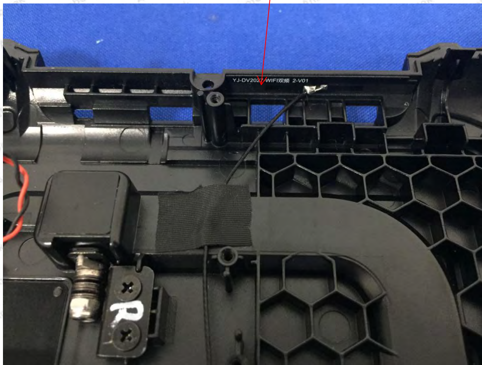
WIFI ANT 2
