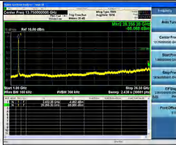
11N40_Ant2_2437_0~Reference
