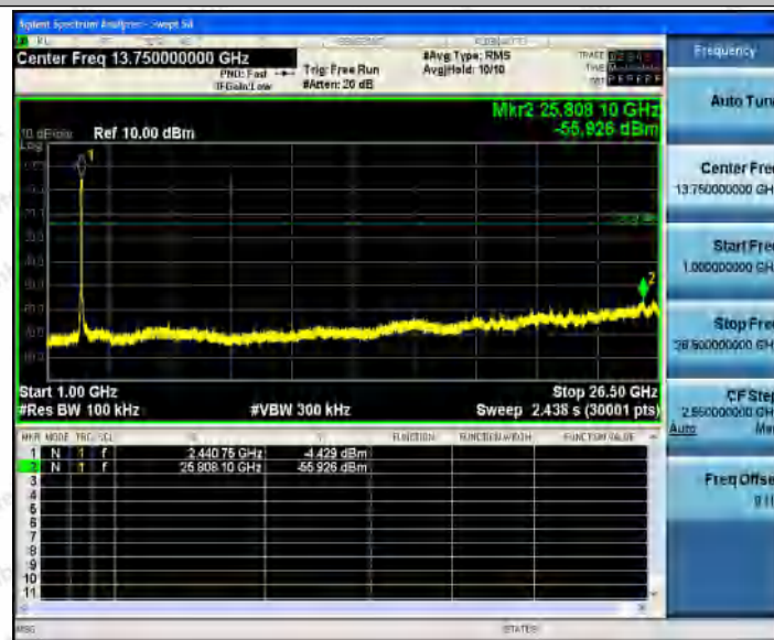
11N40_Ant1_2452_0~Reference
