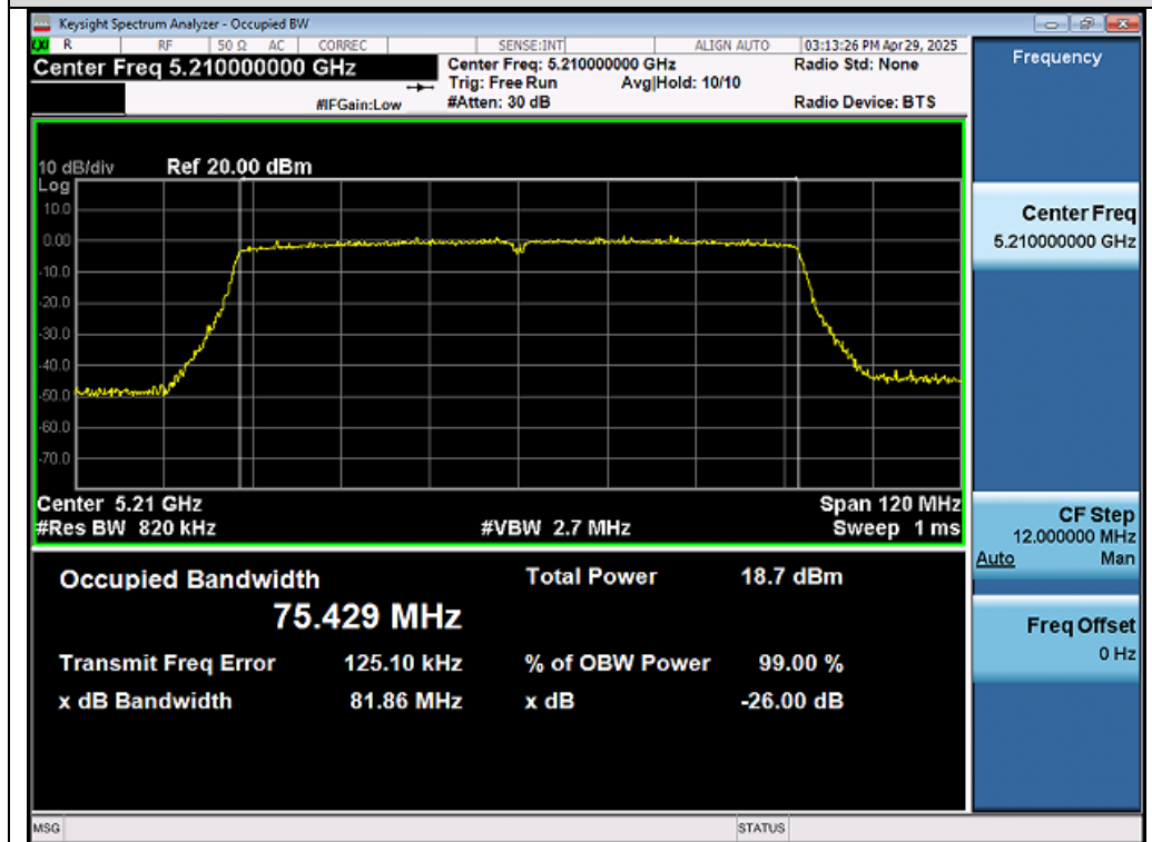
Test_Graph_802.11ac80_Chain B_5210_MCS0_OBW
