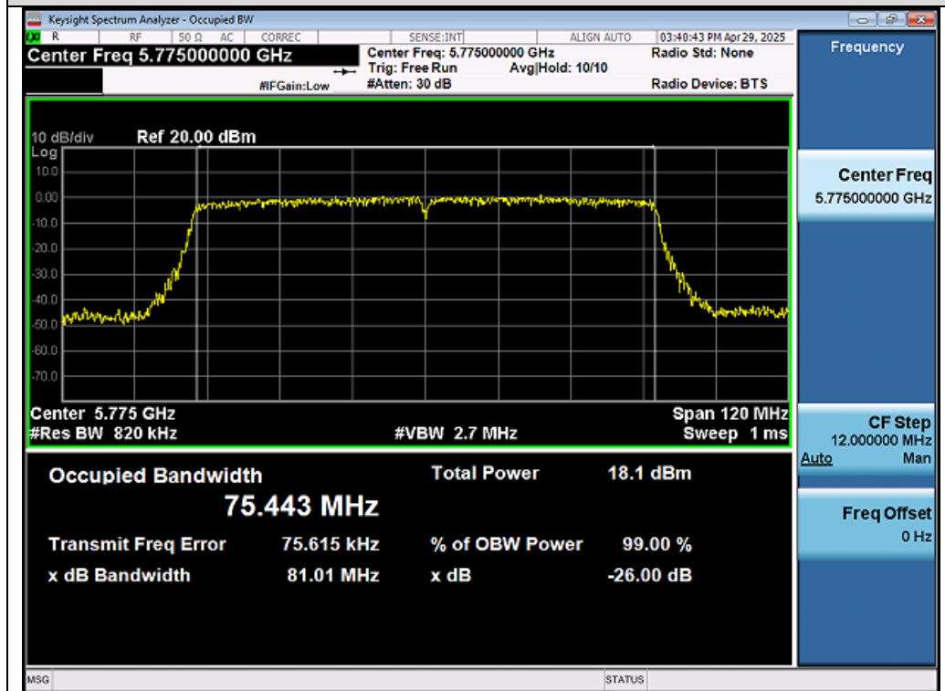
Test_Graph_802.11ac80_Chain B_5775_MCS0_OBW
