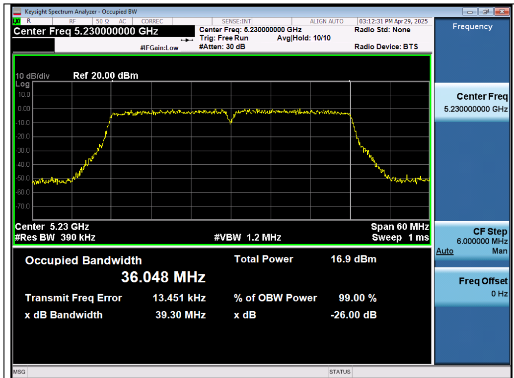
Test_Graph_802.11ac40_Chain B_5230_MCS0_OBW
