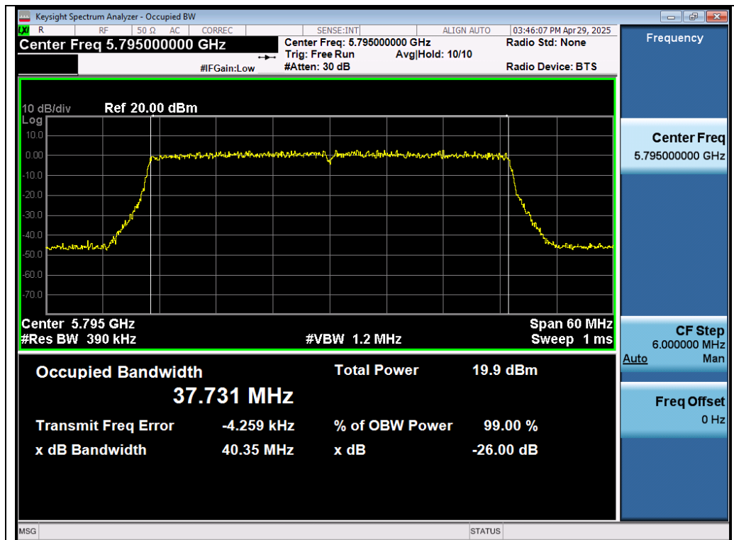
Test_Graph_802.11ax40_Chain B_5795_MCS0_OBW
