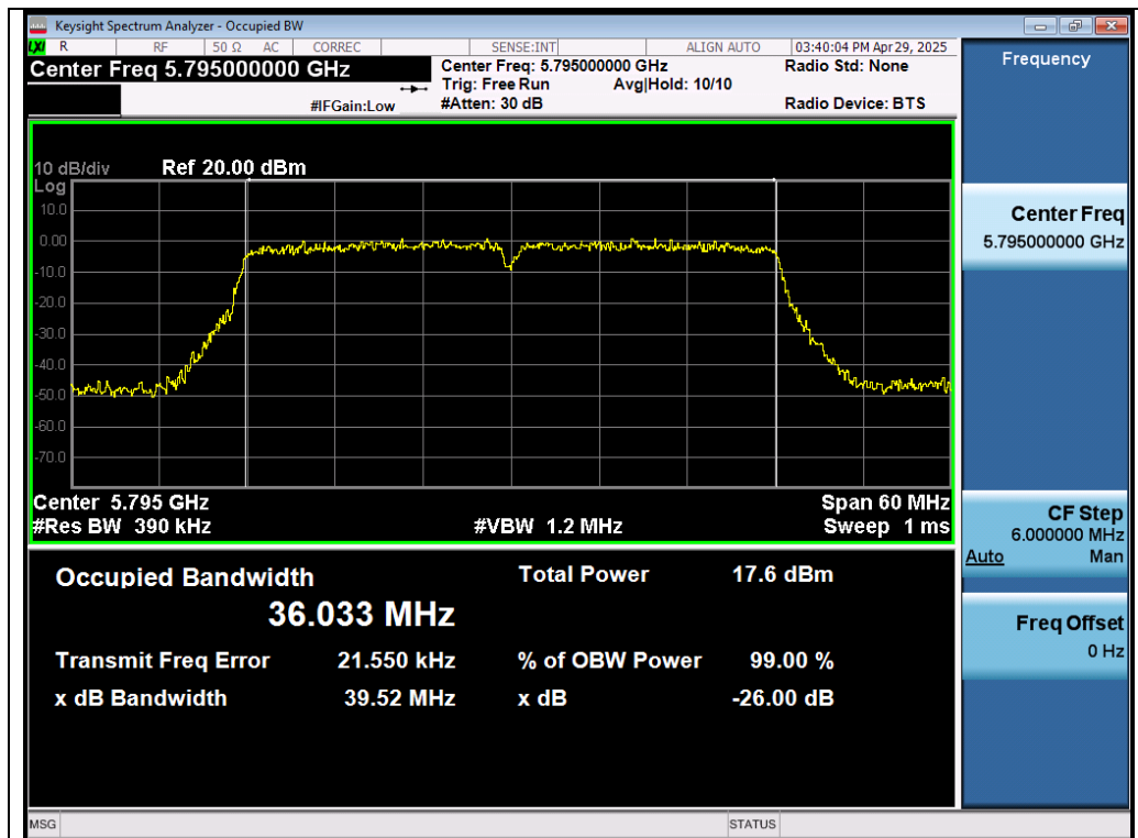
Test_Graph_802.11ac40_Chain B_5795_MCS0_OBW
