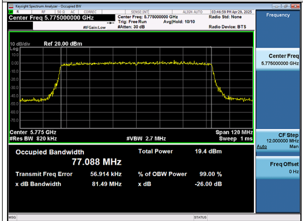
Test_Graph_802.11ax80_Chain B_5775_MCS0_OBW
