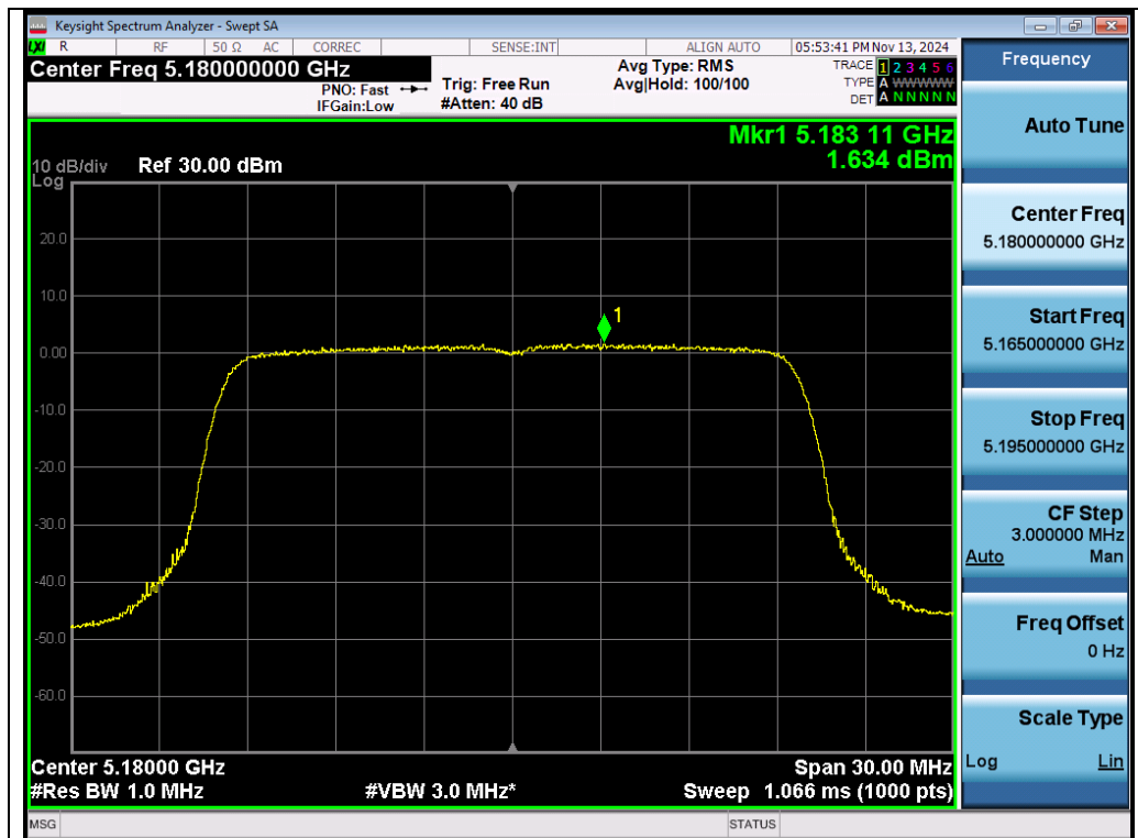
Test_Graph_802.11ax20_Chain B_5180_MCS0_PSD
