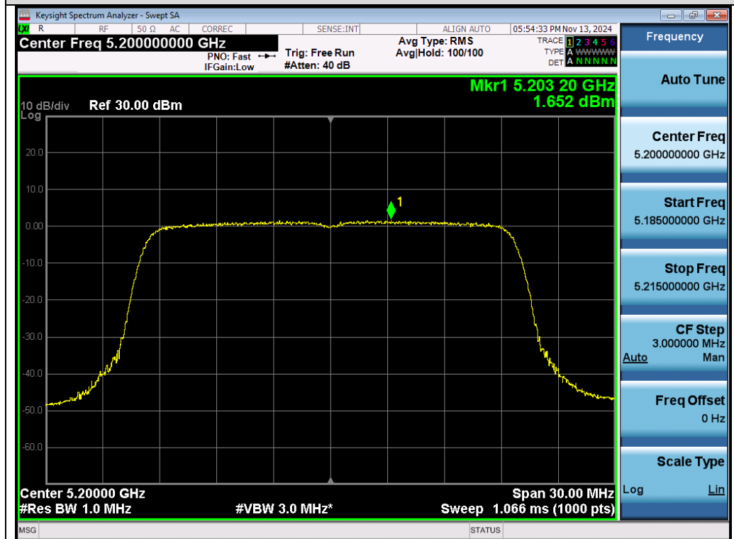
Test_Graph_802.11ax20_Chain B_5200_MCS0_PSD
