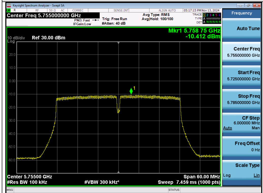
Test_Graph_802.11ac40_Chain A_5755_MCS0_PSD
