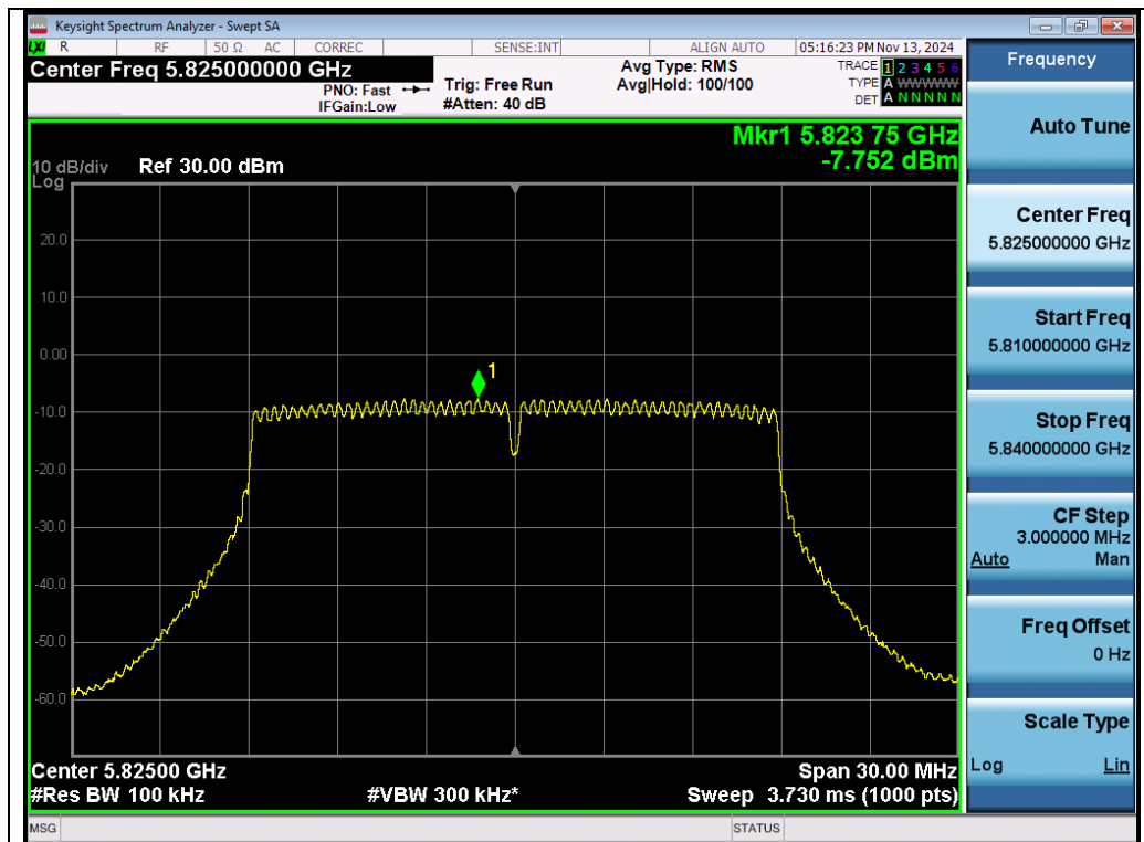
Test_Graph_802.11ac20_Chain A_5825_MCS0_PSD
