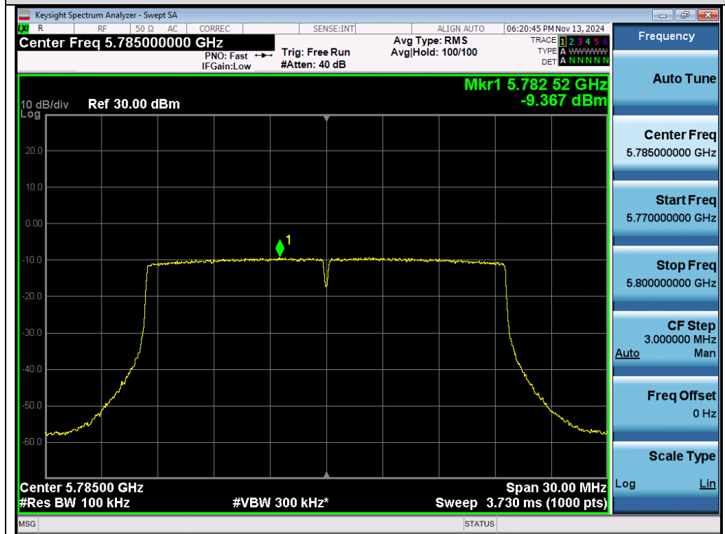
Test_Graph_802.11ax20_Chain B_5785_MCS0_PSD
