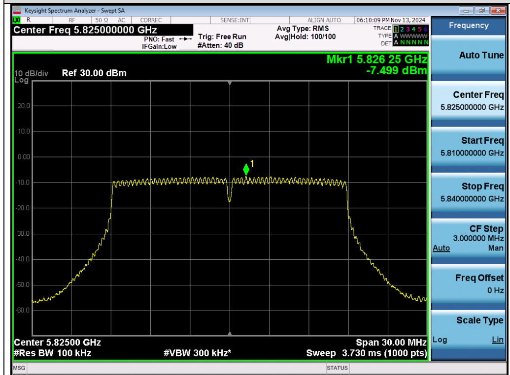
Test_Graph_802.11n20_Chain B_5825_MCS0_PSD
