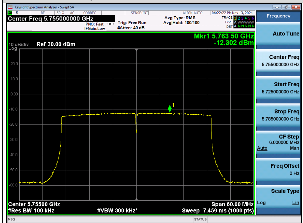
Test_Graph_802.11ax40_Chain B_5755_MCS0_PSD
