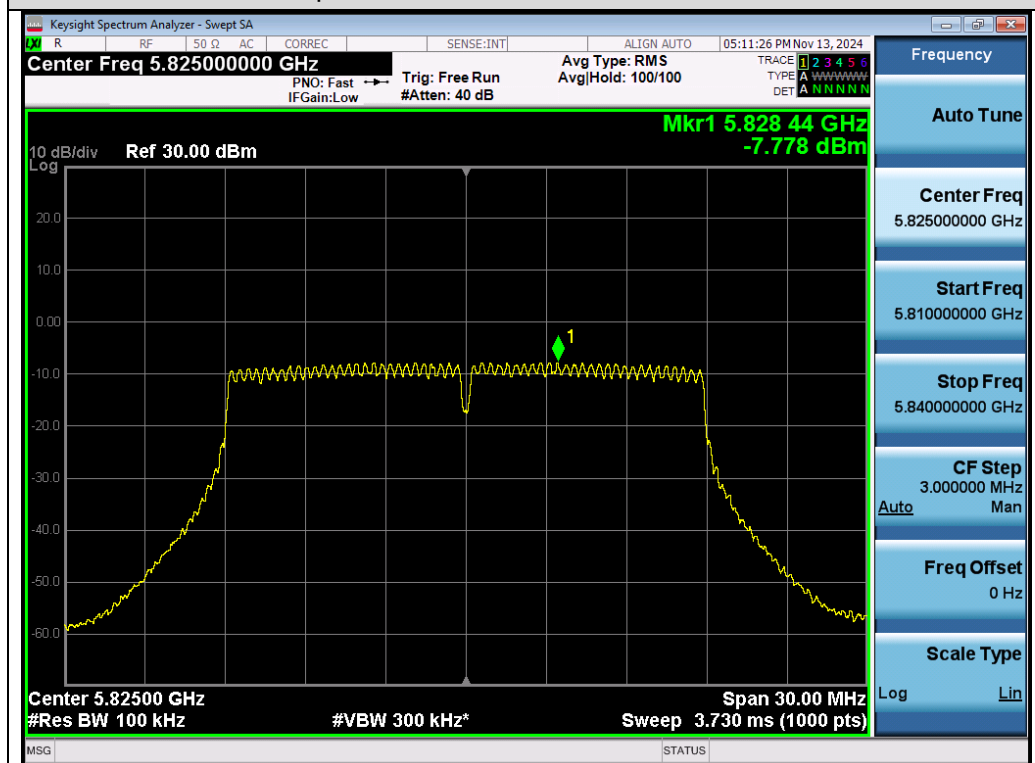
Test_Graph_802.11n20_Chain A_5825_MCS0_PSD
