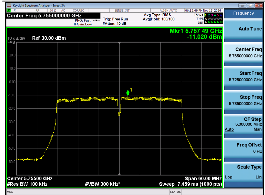
Test_Graph_802.11ac40_Chain B_5755_MCS0_PSD
