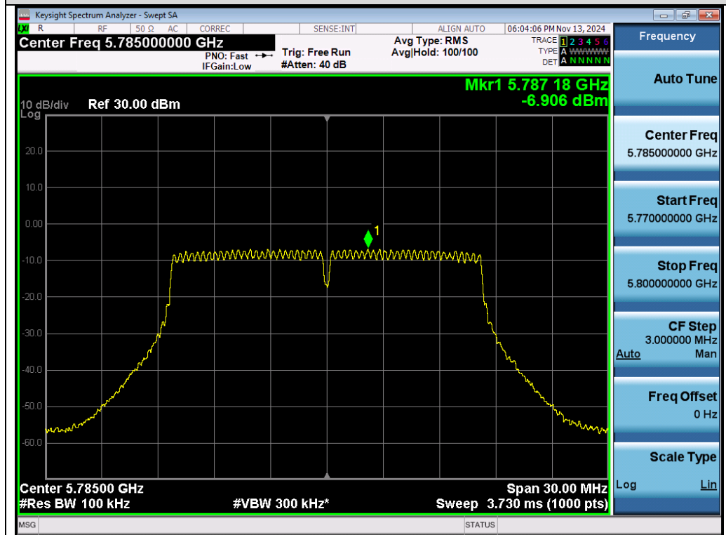
Test_Graph_802.11a_Chain B_5785_6Mbps_PSD
