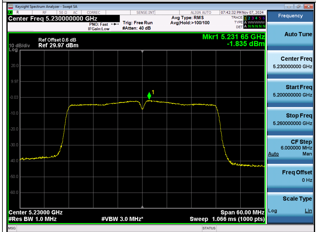
Test_Graph_802.11n40_Chain B_5230_MCS0_PSD
