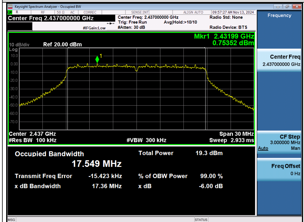
Test_Graph_802.11n20_Chain B_2437_MCS0_DTSBW
