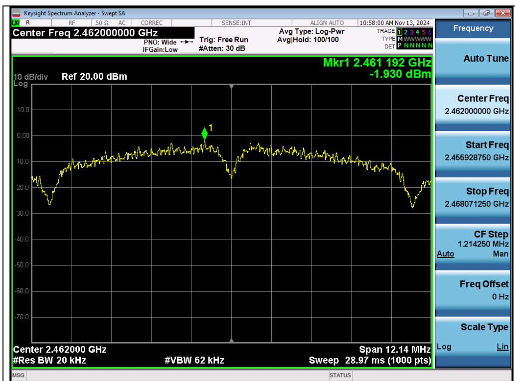
Test_Graph_802.11b_Chain A_2462_1Mbps_PSD
