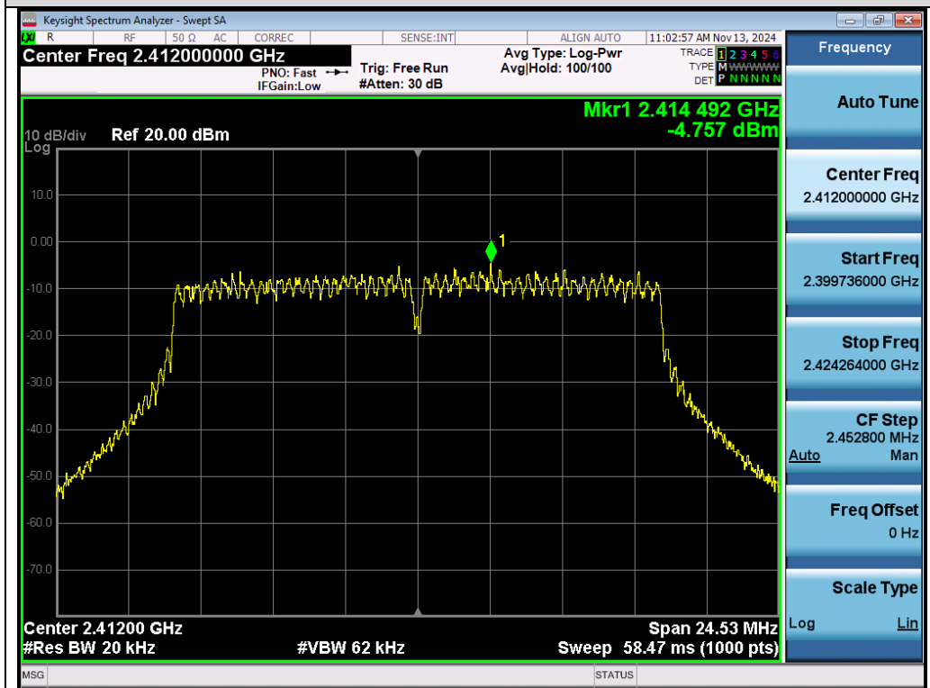
Test_Graph_802.11g_Chain A_2412_6Mbps_PSD
